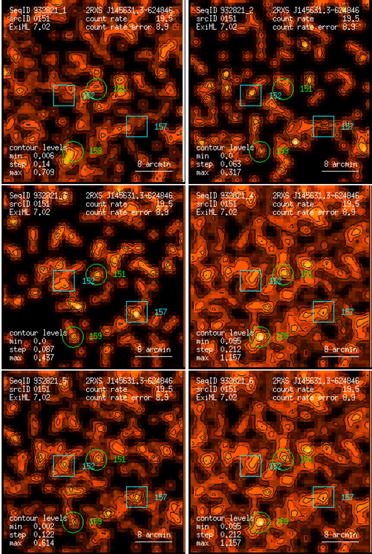
Figure 151: RASS 932821: detection 0151: band rate images, Gaussian filter: (1) PSPC channels 11 – 41, (2) 52 – 90, (3) 91 – 201, (4) 11 – 235, (5) 52 – 201, (6) 11 – 201. Broad band rates in counts/ks. Band rate contour levels in counts/ks/arcmin 2 .
