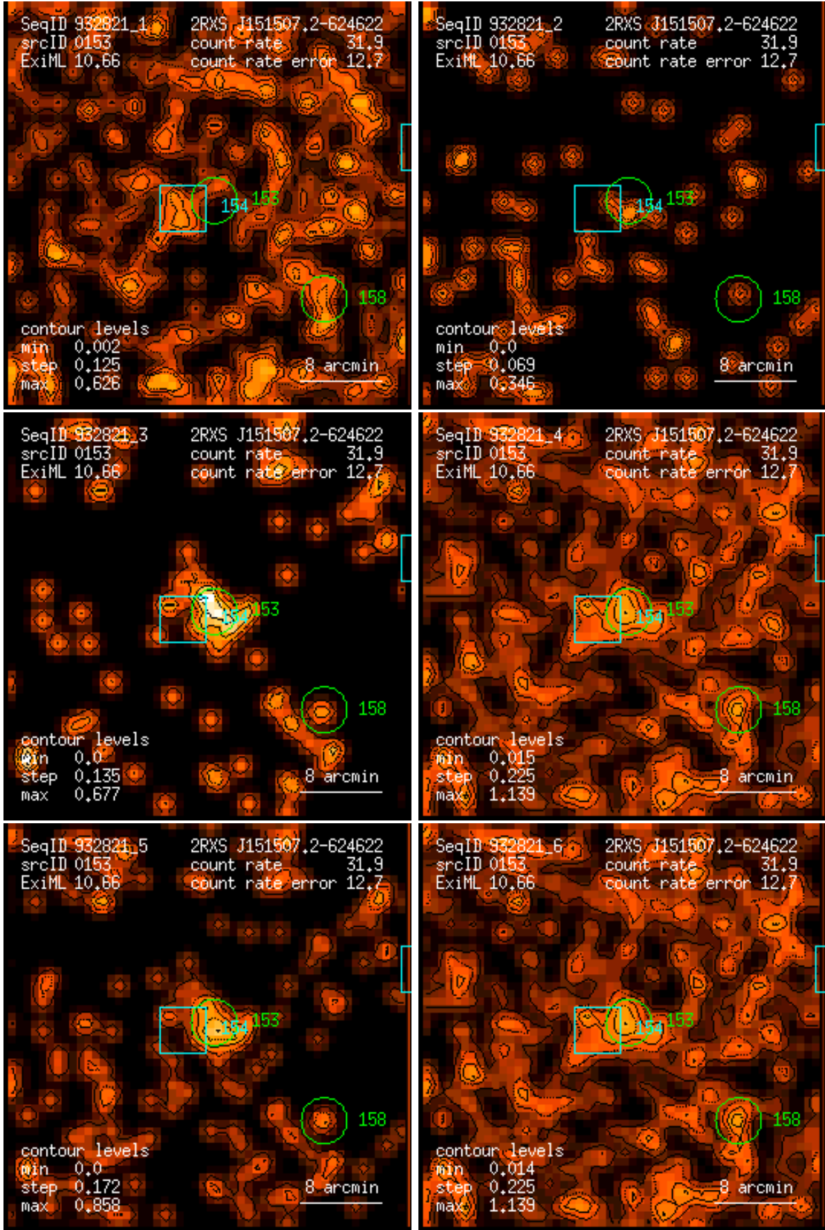
Figure 153: RASS 932821: detection 0153: band rate images, Gaussian filter: (1) PSPC channels 11 – 41, (2) 52 – 90, (3) 91 – 201, (4) 11 – 235, (5) 52 – 201, (6) 11 – 201. Broad band rates in counts/ks. Band rate contour levels in counts/ks/arcmin 2 .
