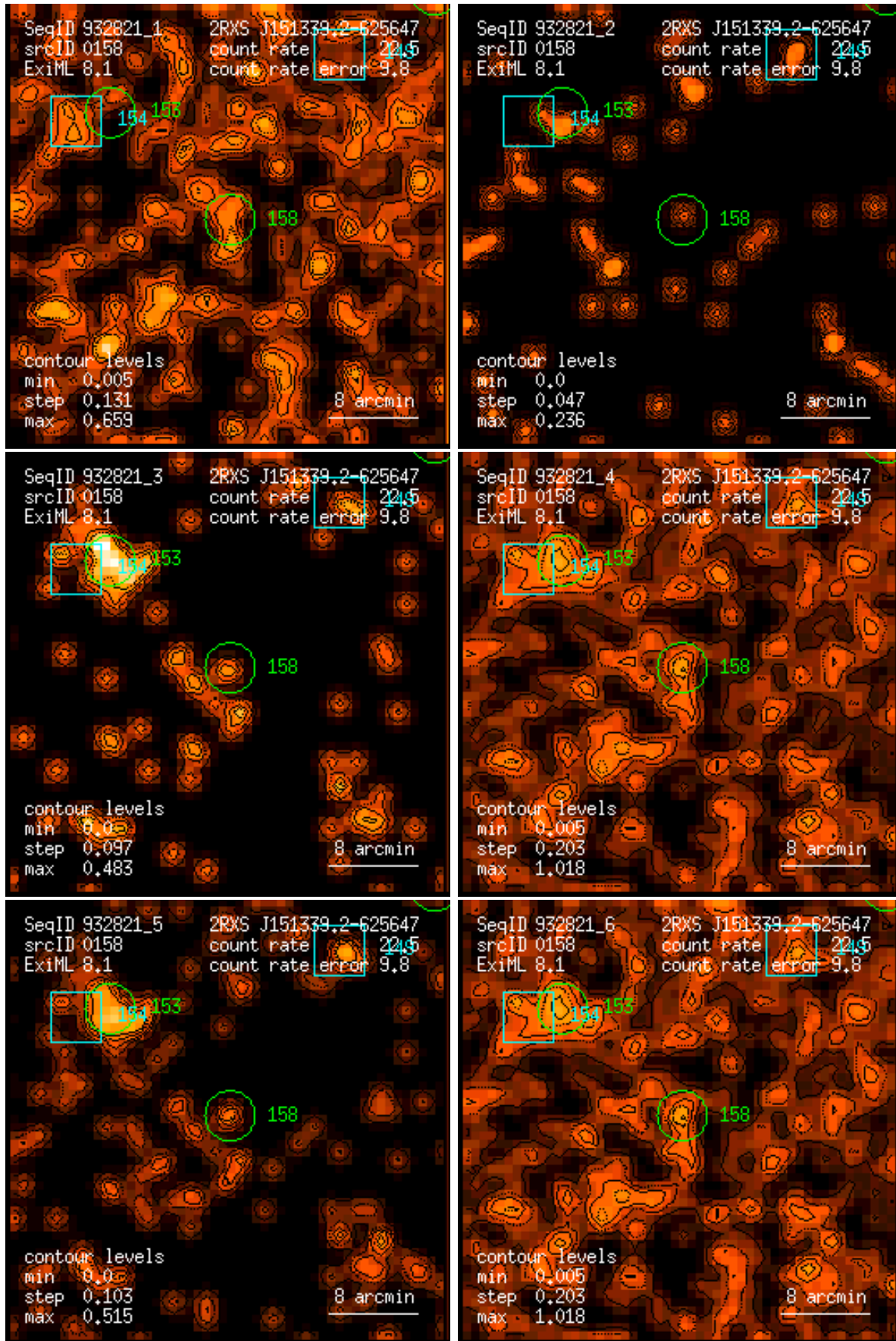
Figure 158: RASS 932821: detection 0158: band rate images, Gaussian filter: (1) PSPC channels 11 – 41, (2) 52 – 90, (3) 91 – 201, (4) 11 – 235, (5) 52 – 201, (6) 11 – 201. Broad band rates in counts/ks. Band rate contour levels in counts/ks/arcmin 2 .
