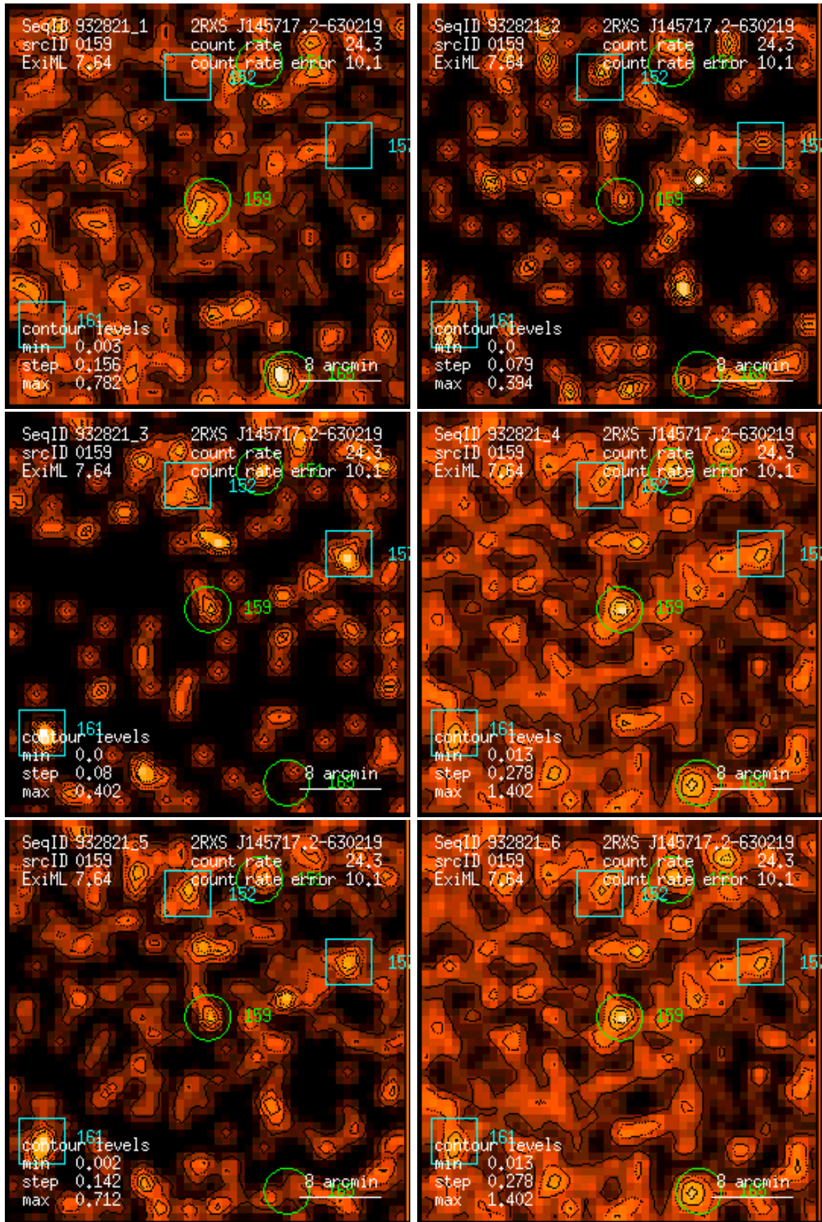
Figure 159: RASS 932821: detection 0159: band rate images, Gaussian filter: (1) PSPC channels 11 – 41, (2) 52 – 90, (3) 91 – 201, (4) 11 – 235, (5) 52 – 201, (6) 11 – 201. Broad band rates in counts/ks. Band rate contour levels in counts/ks/arcmin 2 .
