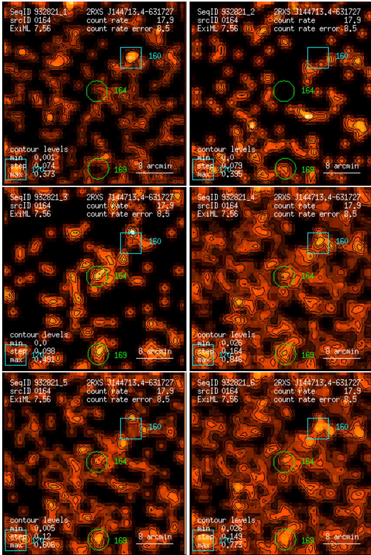
Figure 164: RASS 932821: detection 0164: band rate images, Gaussian filter: (1) PSPC channels 11 – 41, (2) 52 – 90, (3) 91 – 201, (4) 11 – 235, (5) 52 – 201, (6) 11 – 201. Broad band rates in counts/ks. Band rate contour levels in counts/ks/arcmin 2 .
