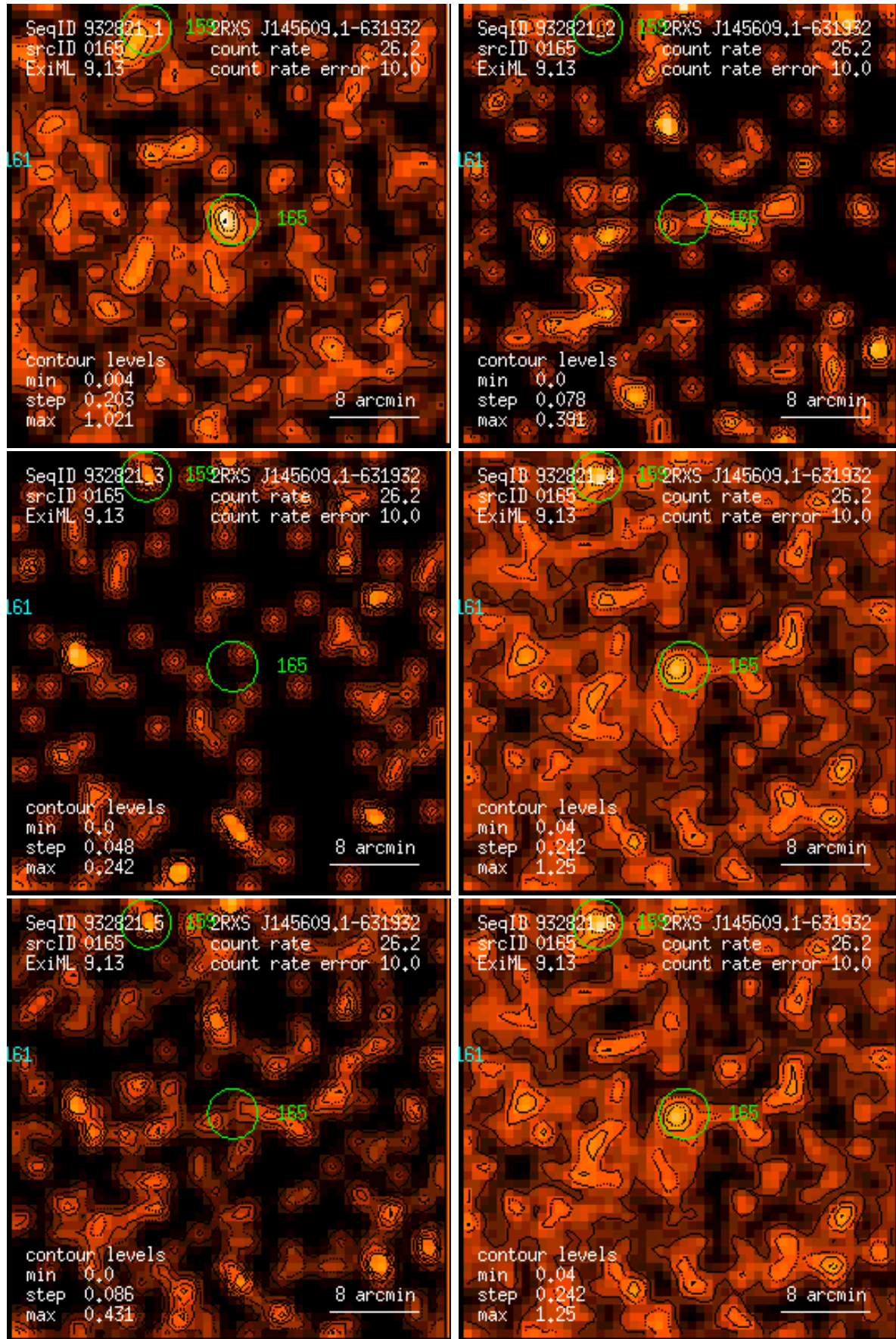
Figure 165: RASS 932821: detection 0165: band rate images, Gaussian filter: (1) PSPC channels 11 – 41, (2) 52 – 90, (3) 91 – 201, (4) 11 – 235, (5) 52 – 201, (6) 11 – 201. Broad band rates in counts/ks. Band rate contour levels in counts/ks/arcmin 2 .
