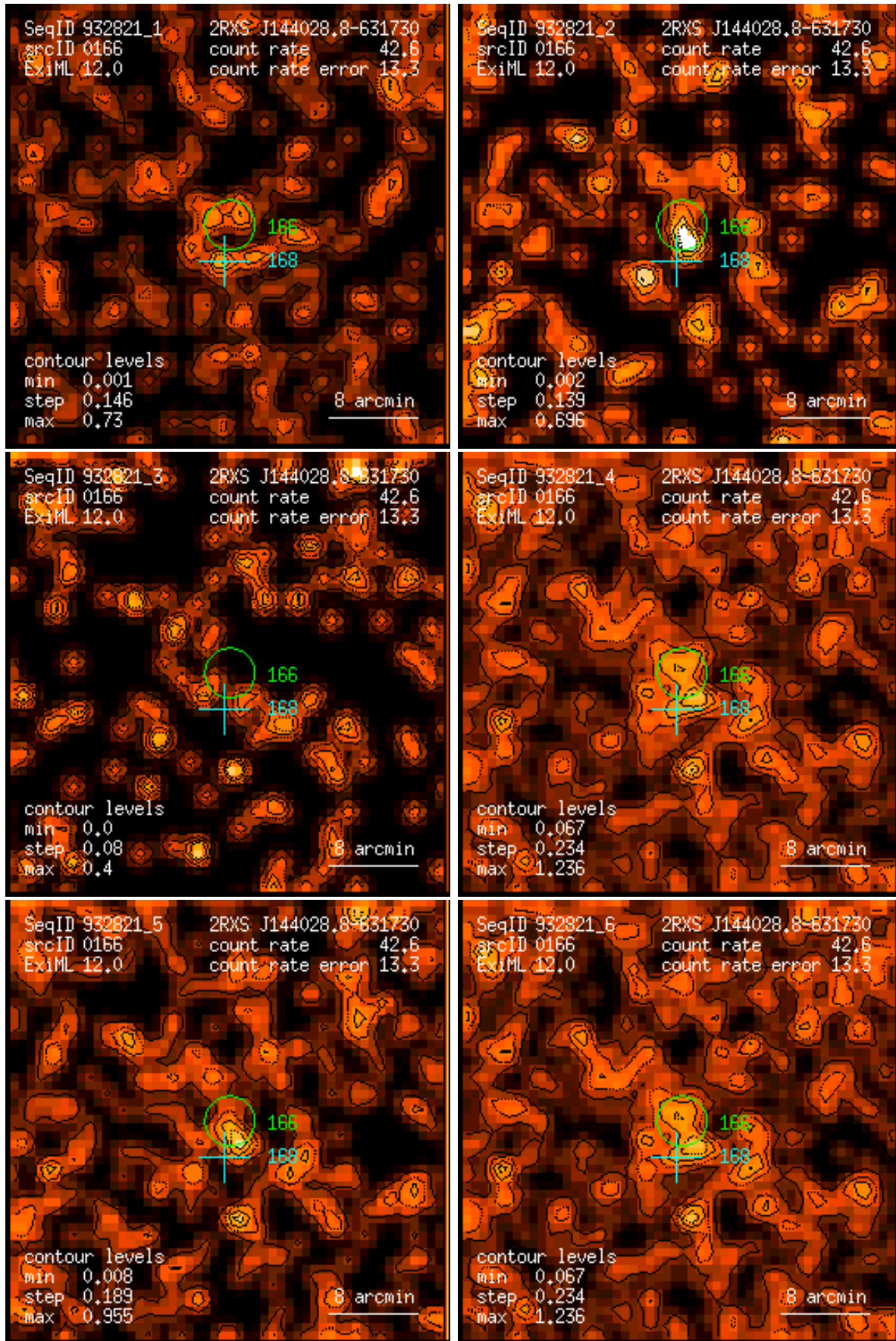
Figure 166: RASS 932821: detection 0166: band rate images, Gaussian filter: (1) PSPC channels 11 – 41, (2) 52 – 90, (3) 91 – 201, (4) 11 – 235, (5) 52 – 201, (6) 11 – 201. Broad band rates in counts/ks. Band rate contour levels in counts/ks/arcmin 2 .
