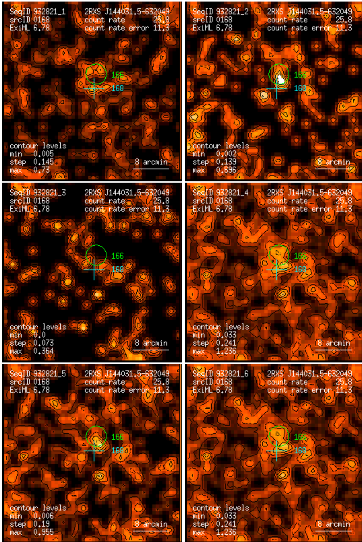
Figure 168: RASS 932821: detection 0168: band rate images, Gaussian filter: (1) PSPC channels 11 – 41, (2) 52 – 90, (3) 91 – 201, (4) 11 – 235, (5) 52 – 201, (6) 11 – 201. Broad band rates in counts/ks. Band rate contour levels in counts/ks/arcmin 2 .
