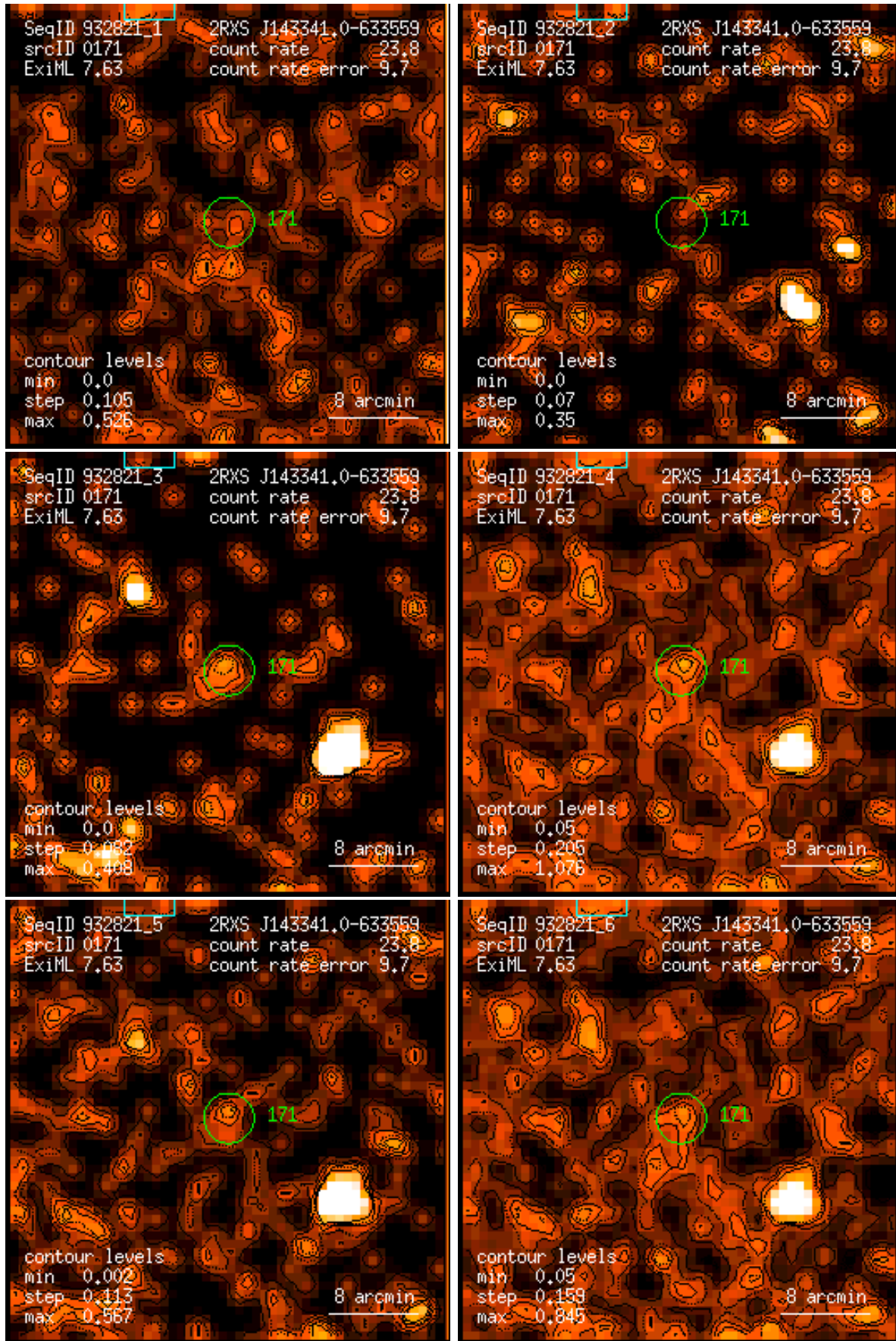
Figure 171: RASS 932821: detection 0171: band rate images, Gaussian filter: (1) PSPC channels 11 – 41, (2) 52 – 90, (3) 91 – 201, (4) 11 – 235, (5) 52 – 201, (6) 11 – 201. Broad band rates in counts/ks. Band rate contour levels in counts/ks/arcmin 2 .
