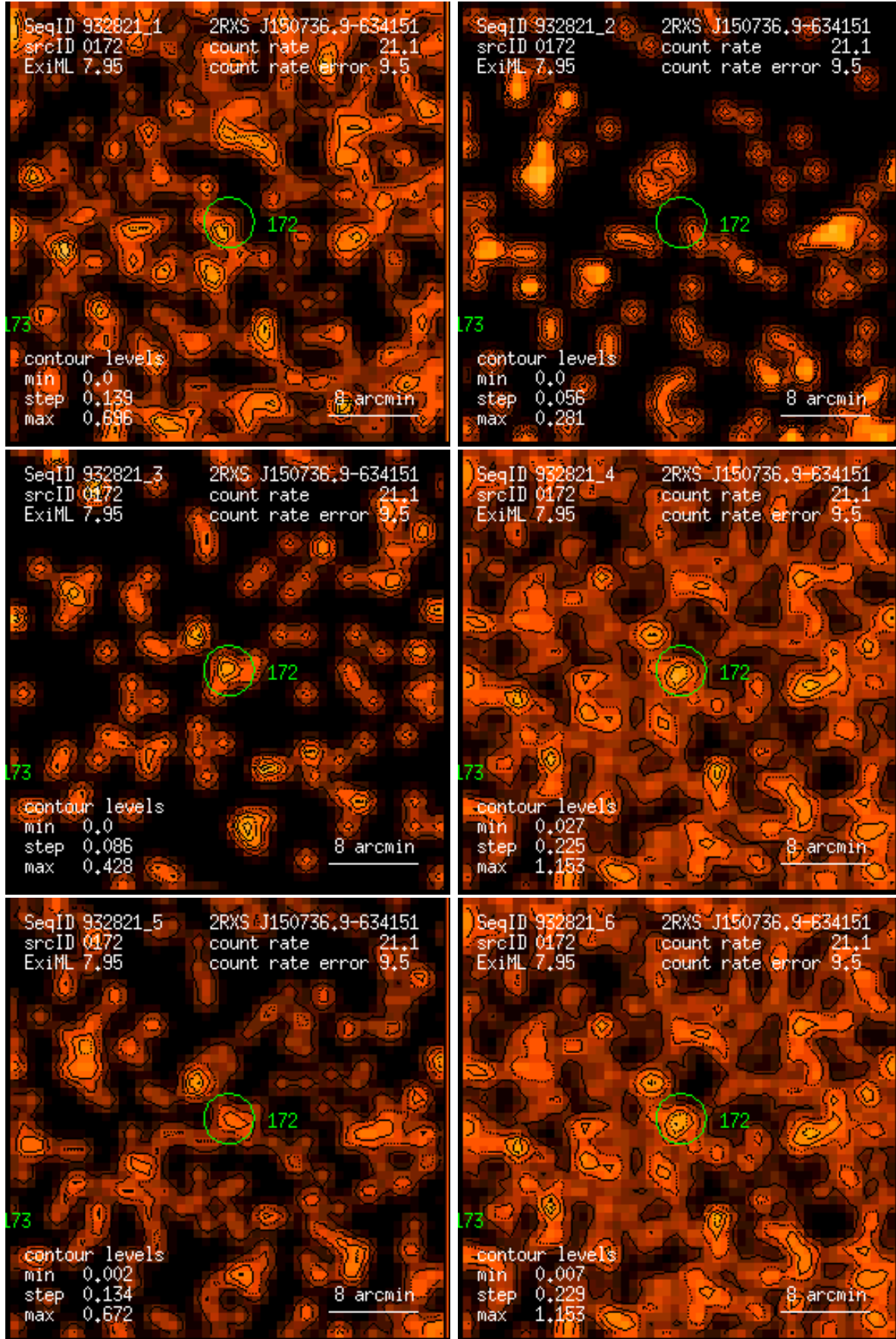
Figure 172: RASS 932821: detection 0172: band rate images, Gaussian filter: (1) PSPC channels 11 – 41, (2) 52 – 90, (3) 91 – 201, (4) 11 – 235, (5) 52 – 201, (6) 11 – 201. Broad band rates in counts/ks. Band rate contour levels in counts/ks/arcmin 2 .
