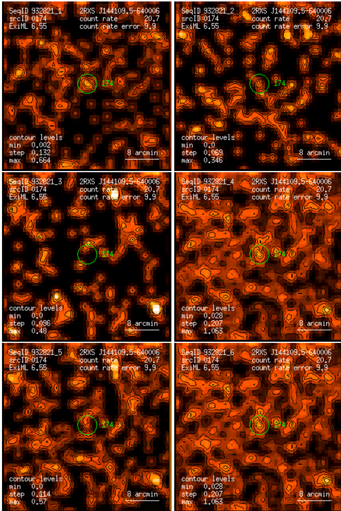
Figure 174: RASS 932821: detection 0174: band rate images, Gaussian filter: (1) PSPC channels 11 – 41, (2) 52 – 90, (3) 91 – 201, (4) 11 – 235, (5) 52 – 201, (6) 11 – 201. Broad band rates in counts/ks. Band rate contour levels in counts/ks/arcmin 2 .
