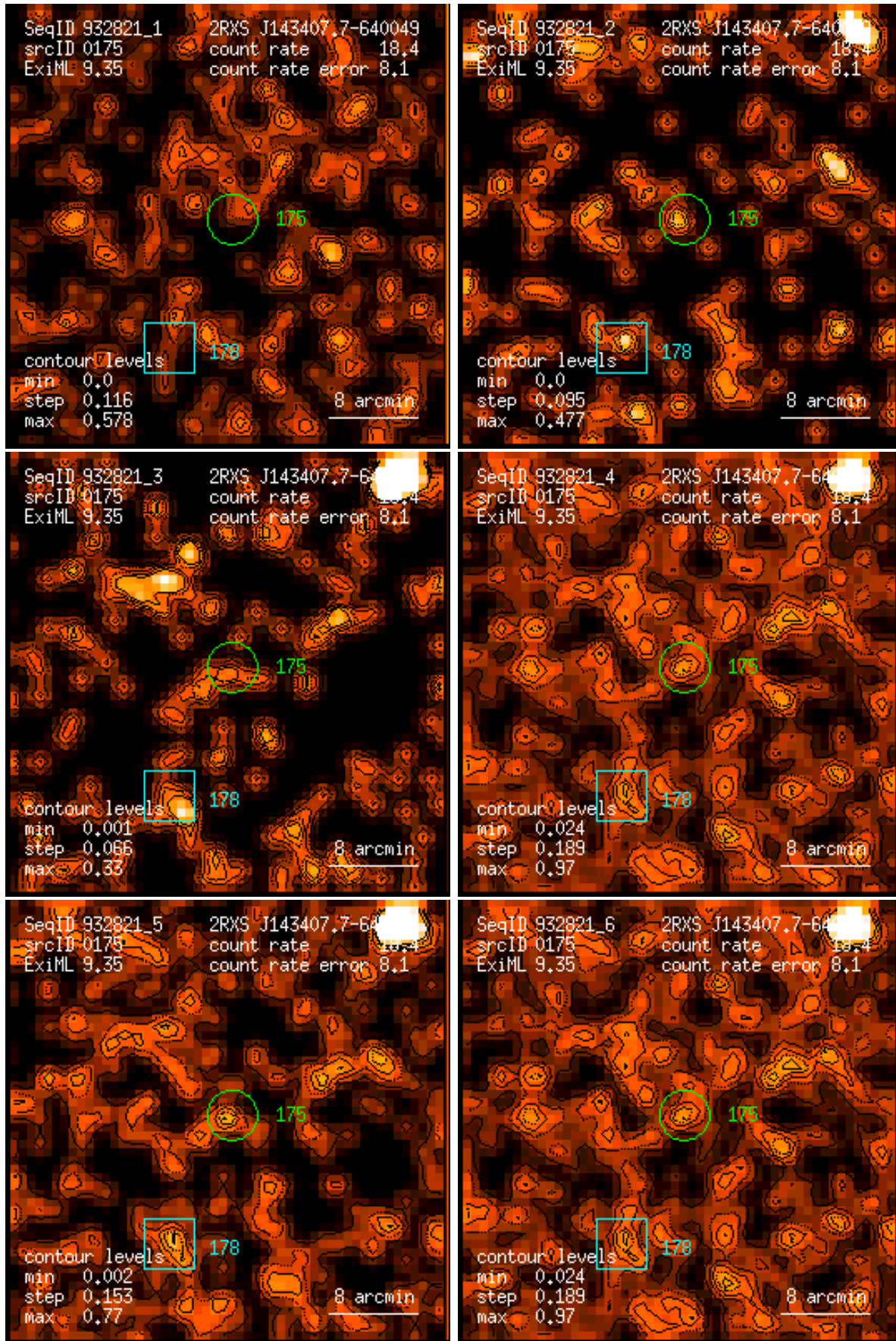
Figure 175: RASS 932821: detection 0175: band rate images, Gaussian filter: (1) PSPC channels 11 – 41, (2) 52 – 90, (3) 91 – 201, (4) 11 – 235, (5) 52 – 201, (6) 11 – 201. Broad band rates in counts/ks. Band rate contour levels in counts/ks/arcmin 2 .
