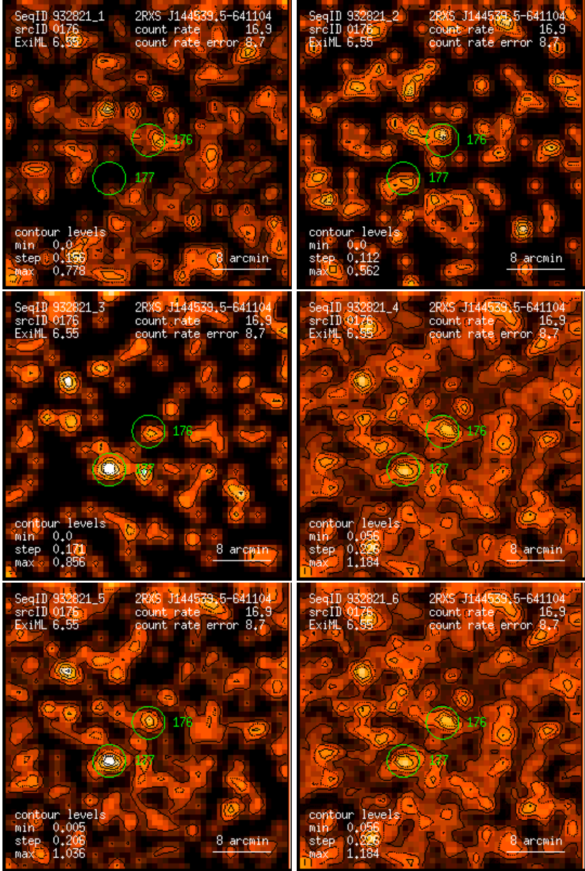
Figure 176: RASS 932821: detection 0176: band rate images, Gaussian filter: (1) PSPC channels 11 – 41, (2) 52 – 90, (3) 91 – 201, (4) 11 – 235, (5) 52 – 201, (6) 11 – 201. Broad band rates in counts/ks. Band rate contour levels in counts/ks/arcmin 2 .
