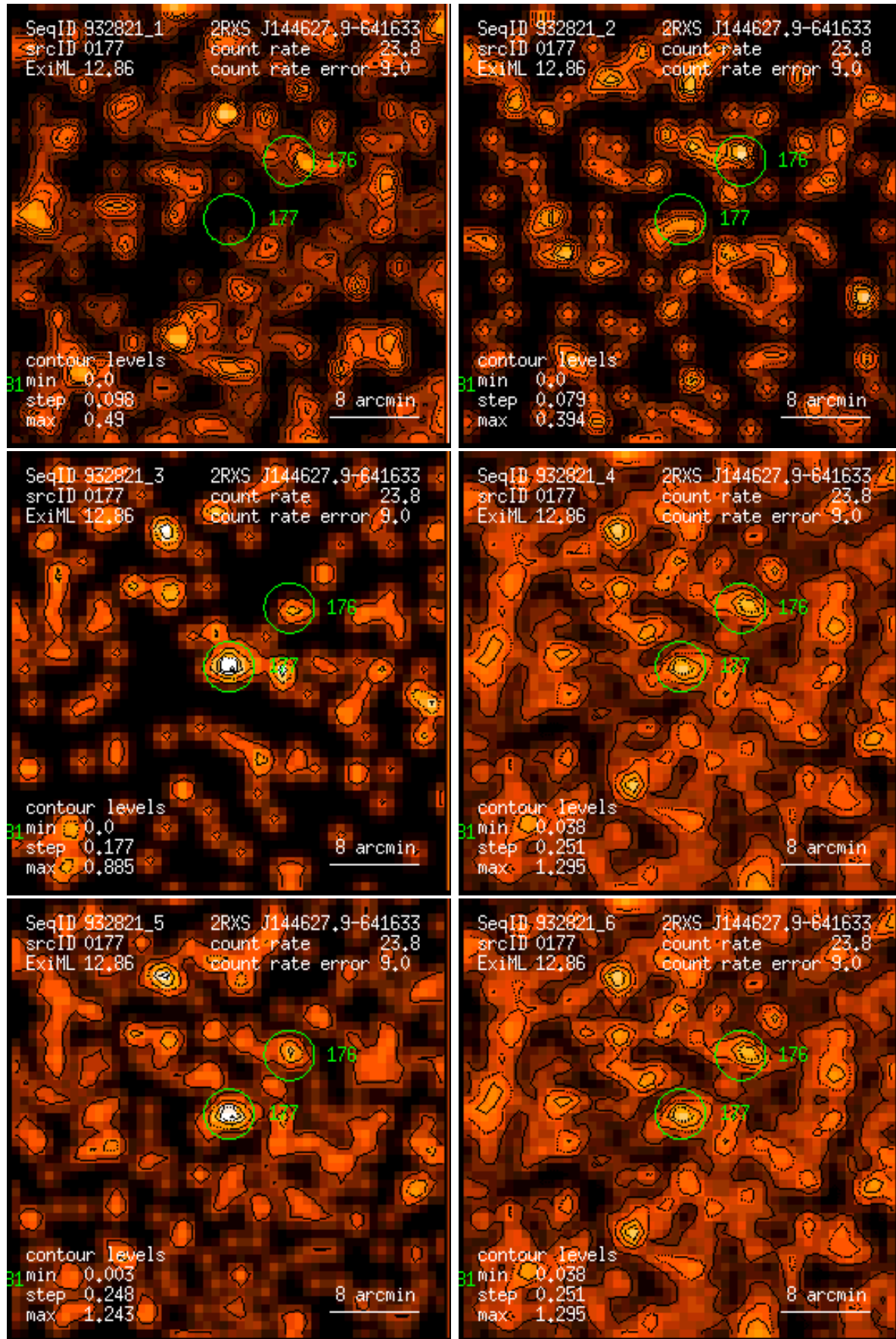
Figure 177: RASS 932821: detection 0177: band rate images, Gaussian filter: (1) PSPC channels 11 – 41, (2) 52 – 90, (3) 91 – 201, (4) 11 – 235, (5) 52 – 201, (6) 11 – 201. Broad band rates in counts/ks. Band rate contour levels in counts/ks/arcmin 2 .
