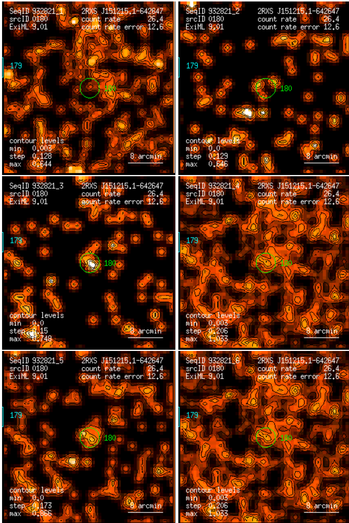
Figure 180: RASS 932821: detection 0180: band rate images, Gaussian filter: (1) PSPC channels 11 – 41, (2) 52 – 90, (3) 91 – 201, (4) 11 – 235, (5) 52 – 201, (6) 11 – 201. Broad band rates in counts/ks. Band rate contour levels in counts/ks/arcmin 2 .
