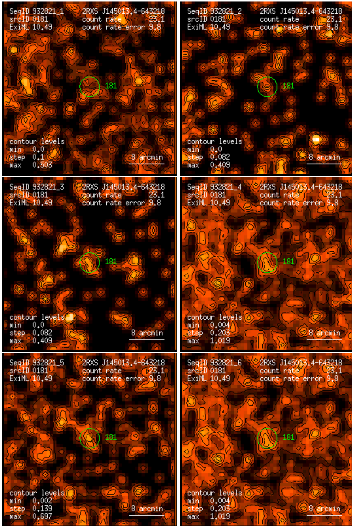
Figure 181: RASS 932821: detection 0181: band rate images, Gaussian filter: (1) PSPC channels 11 – 41, (2) 52 – 90, (3) 91 – 201, (4) 11 – 235, (5) 52 – 201, (6) 11 – 201. Broad band rates in counts/ks. Band rate contour levels in counts/ks/arcmin 2 .
