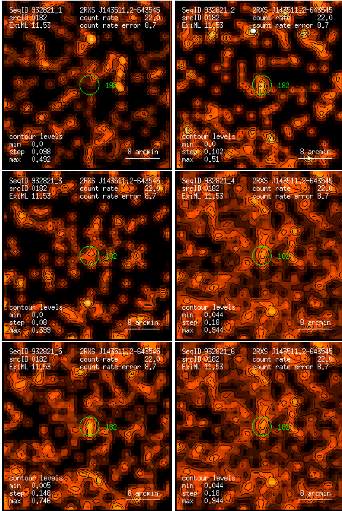
Figure 182: RASS 932821: detection 0182: band rate images, Gaussian filter: (1) PSPC channels 11 – 41, (2) 52 – 90, (3) 91 – 201, (4) 11 – 235, (5) 52 – 201, (6) 11 – 201. Broad band rates in counts/ks. Band rate contour levels in counts/ks/arcmin 2 .
