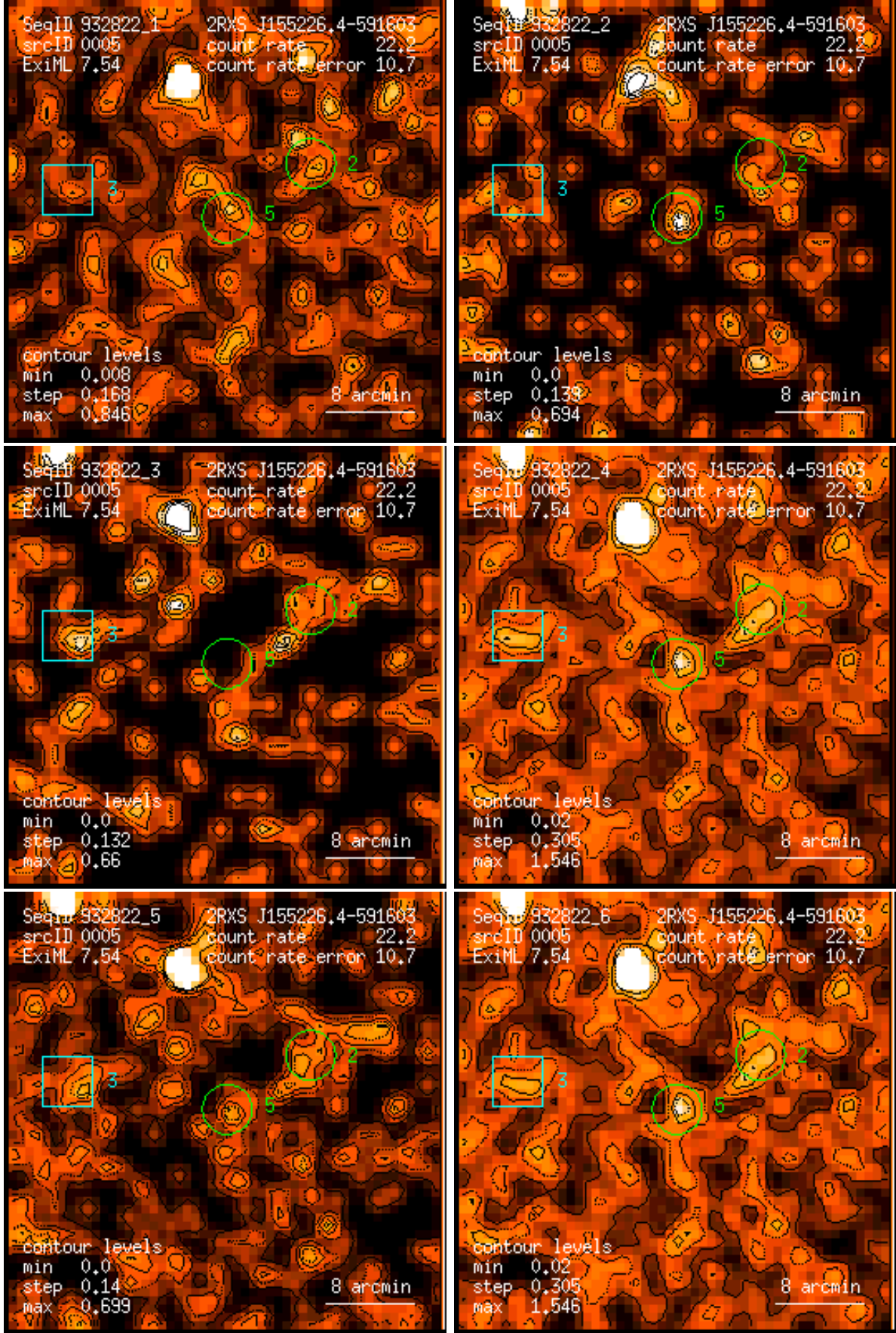
Figure 5: RASS 932822: detection 0005: band rate images, Gaussian filter: (1) PSPC channels 11 – 41, (2) 52 – 90, (3) 91 – 201, (4) 11 – 235, (5) 52 – 201, (6) 11 – 201. Broad band rates in counts/ks. Band rate contour levels in counts/ks/arcmin 2 .
