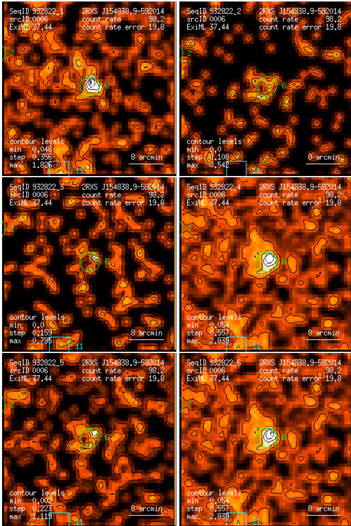
Figure 6: RASS 932822: detection 0006: band rate images, Gaussian filter: (1) PSPC channels 11 – 41, (2) 52 – 90, (3) 91 – 201, (4) 11 – 235, (5) 52 – 201, (6) 11 – 201. Broad band rates in counts/ks. Band rate contour levels in counts/ks/arcmin 2 .
