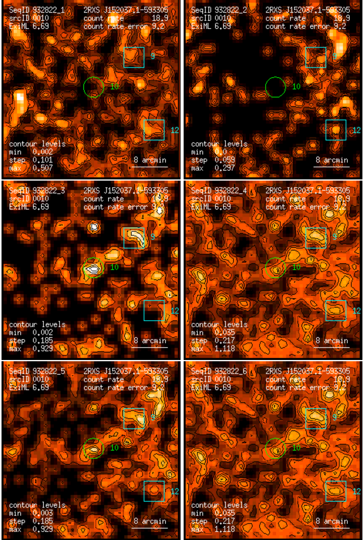
Figure 10: RASS 932822: detection 0010: band rate images, Gaussian filter: (1) PSPC channels 11 – 41, (2) 52 – 90, (3) 91 – 201, (4) 11 – 235, (5) 52 – 201, (6) 11 – 201. Broad band rates in counts/ks. Band rate contour levels in counts/ks/arcmin 2 .
