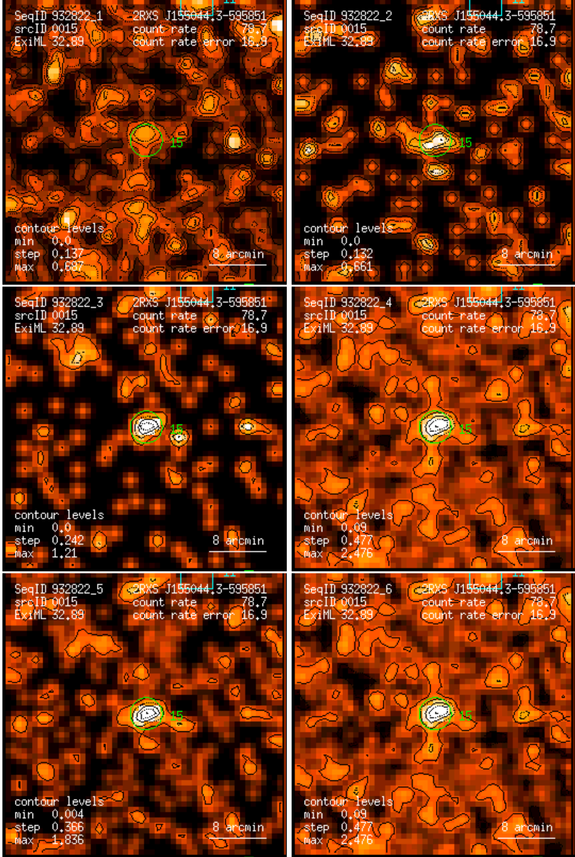
Figure 15: RASS 932822: detection 0015: band rate images, Gaussian filter: (1) PSPC channels 11 – 41, (2) 52 – 90, (3) 91 – 201, (4) 11 – 235, (5) 52 – 201, (6) 11 – 201. Broad band rates in counts/ks. Band rate contour levels in counts/ks/arcmin 2 .
