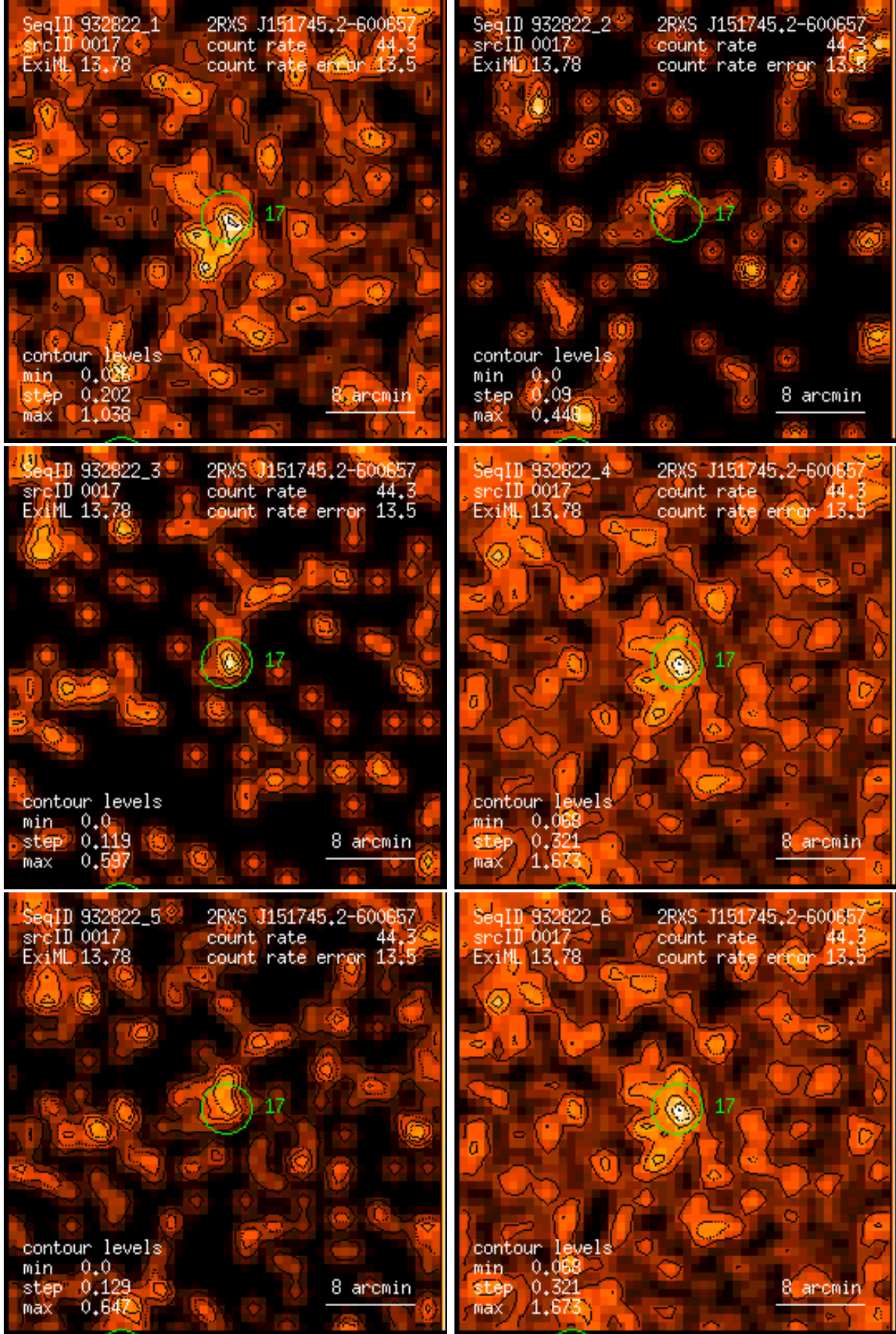
Figure 17: RASS 932822: detection 0017: band rate images, Gaussian filter: (1) PSPC channels 11 – 41, (2) 52 – 90, (3) 91 – 201, (4) 11 – 235, (5) 52 – 201, (6) 11 – 201. Broad band rates in counts/ks. Band rate contour levels in counts/ks/arcmin 2 .
