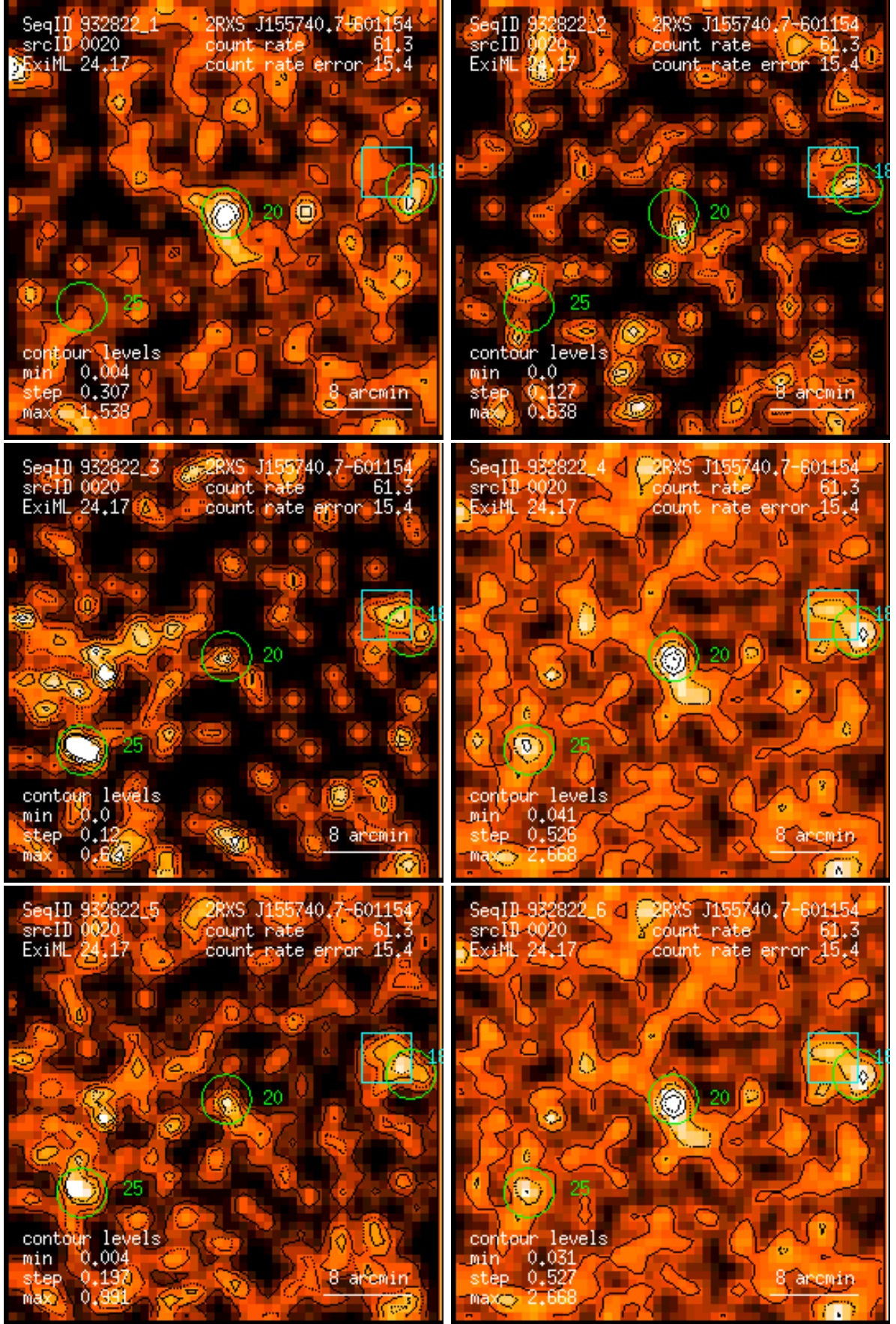
Figure 20: RASS 932822: detection 0020: band rate images, Gaussian filter: (1) PSPC channels 11 – 41, (2) 52 – 90, (3) 91 – 201, (4) 11 – 235, (5) 52 – 201, (6) 11 – 201. Broad band rates in counts/ks. Band rate contour levels in counts/ks/arcmin 2 .
