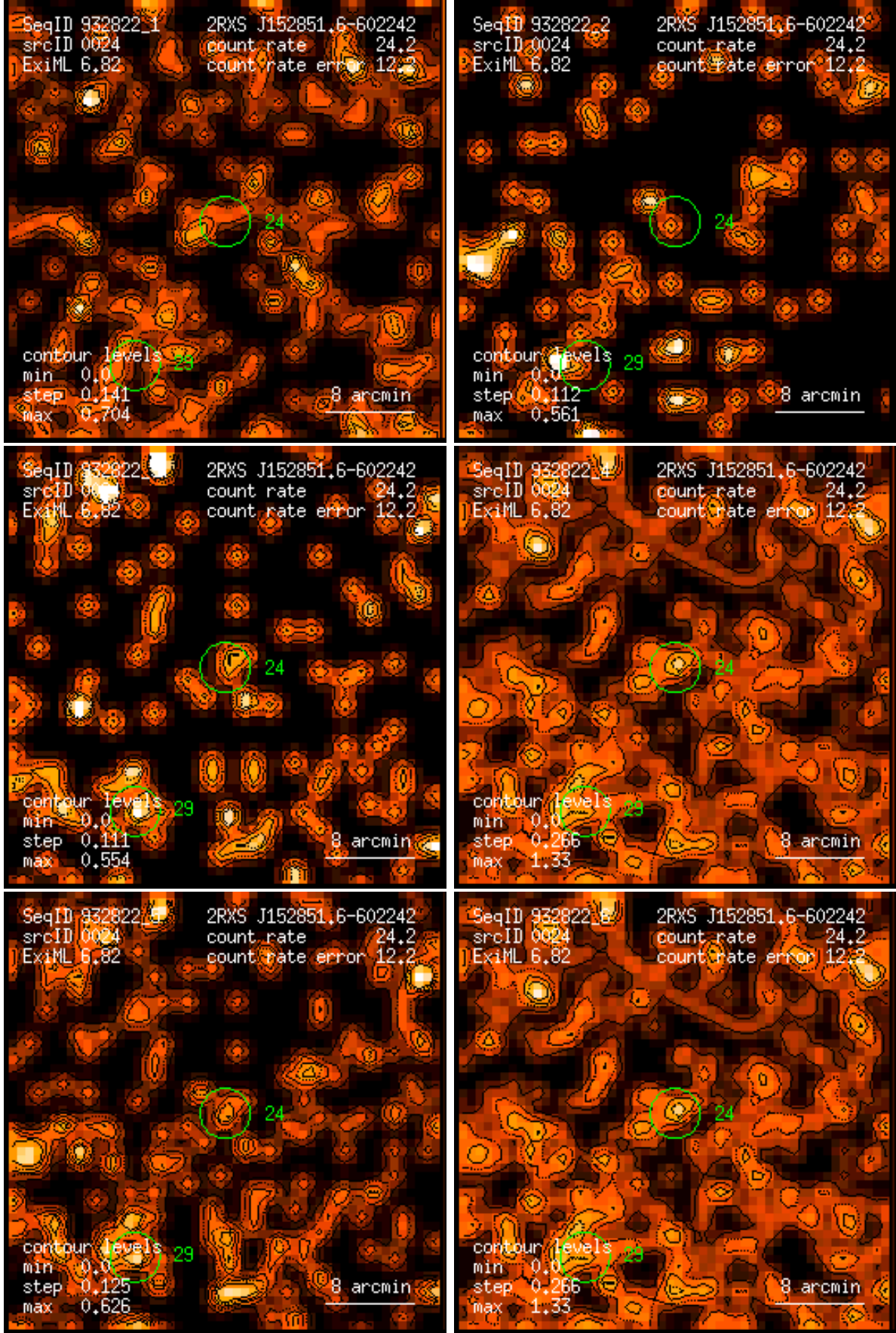
Figure 24: RASS 932822: detection 0024: band rate images, Gaussian filter: (1) PSPC channels 11 – 41, (2) 52 – 90, (3) 91 – 201, (4) 11 – 235, (5) 52 – 201, (6) 11 – 201. Broad band rates in counts/ks. Band rate contour levels in counts/ks/arcmin 2 .
