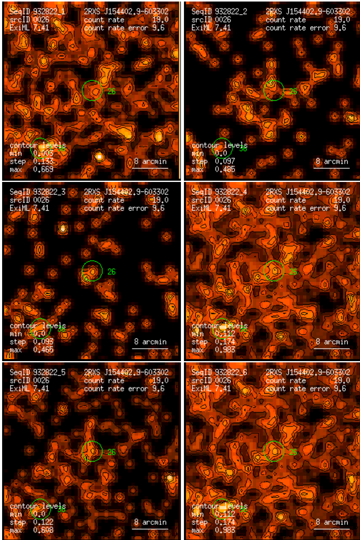
Figure 26: RASS 932822: detection 0026: band rate images, Gaussian filter: (1) PSPC channels 11 – 41, (2) 52 – 90, (3) 91 – 201, (4) 11 – 235, (5) 52 – 201, (6) 11 – 201. Broad band rates in counts/ks. Band rate contour levels in counts/ks/arcmin 2 .
