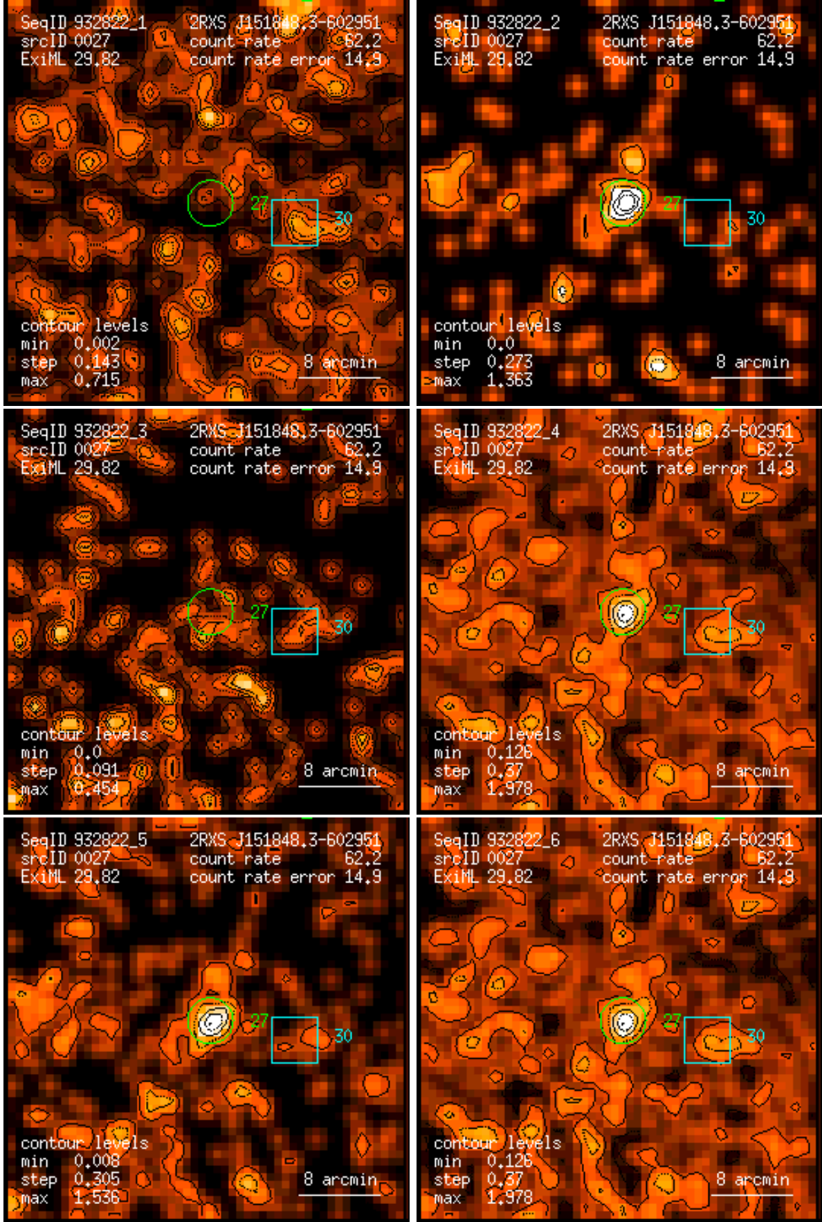
Figure 27: RASS 932822: detection 0027: band rate images, Gaussian filter: (1) PSPC channels 11 – 41, (2) 52 – 90, (3) 91 – 201, (4) 11 – 235, (5) 52 – 201, (6) 11 – 201. Broad band rates in counts/ks. Band rate contour levels in counts/ks/arcmin 2 .
