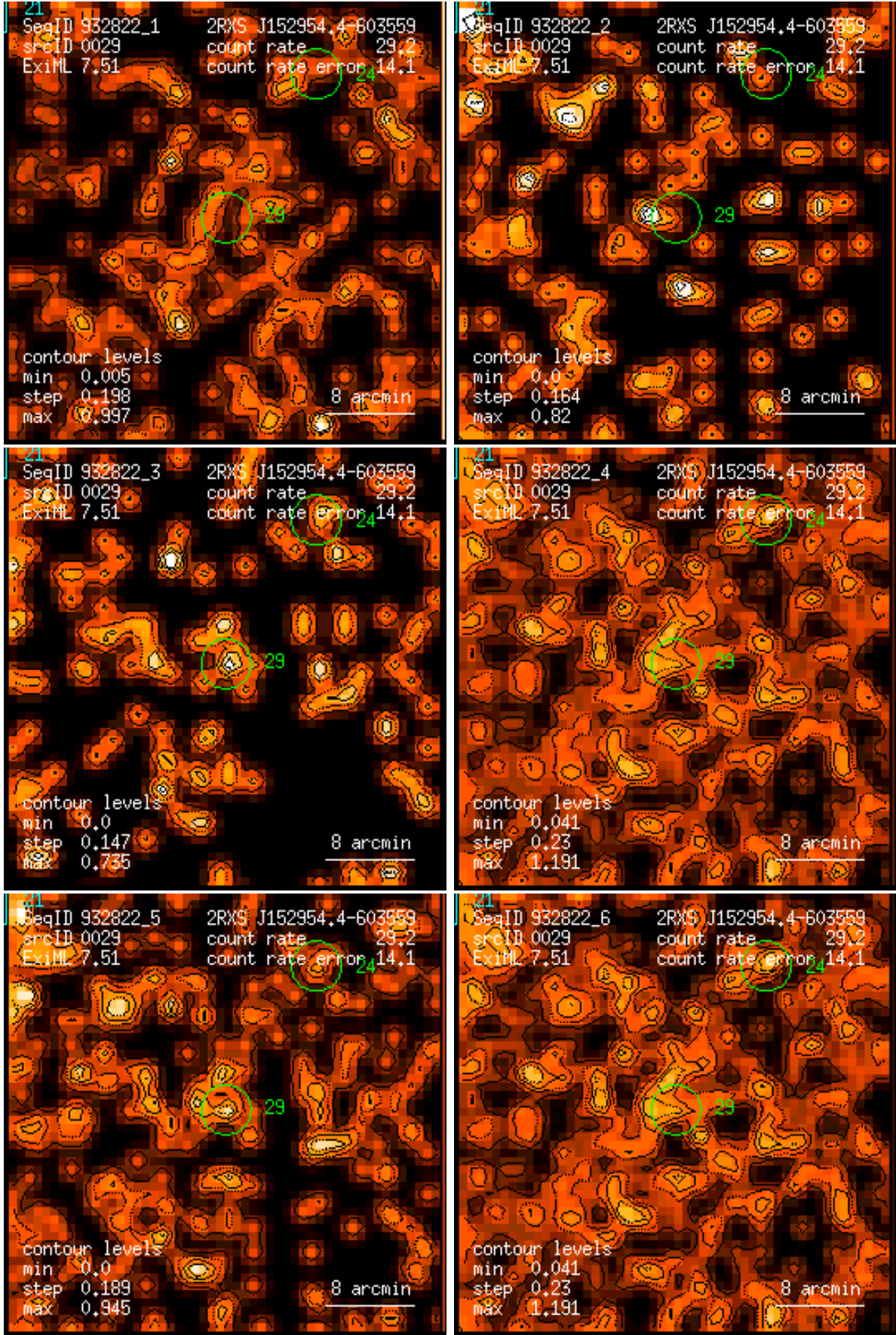
Figure 29: RASS 932822: detection 0029: band rate images, Gaussian filter: (1) PSPC channels 11 – 41, (2) 52 – 90, (3) 91 – 201, (4) 11 – 235, (5) 52 – 201, (6) 11 – 201. Broad band rates in counts/ks. Band rate contour levels in counts/ks/arcmin 2 .
