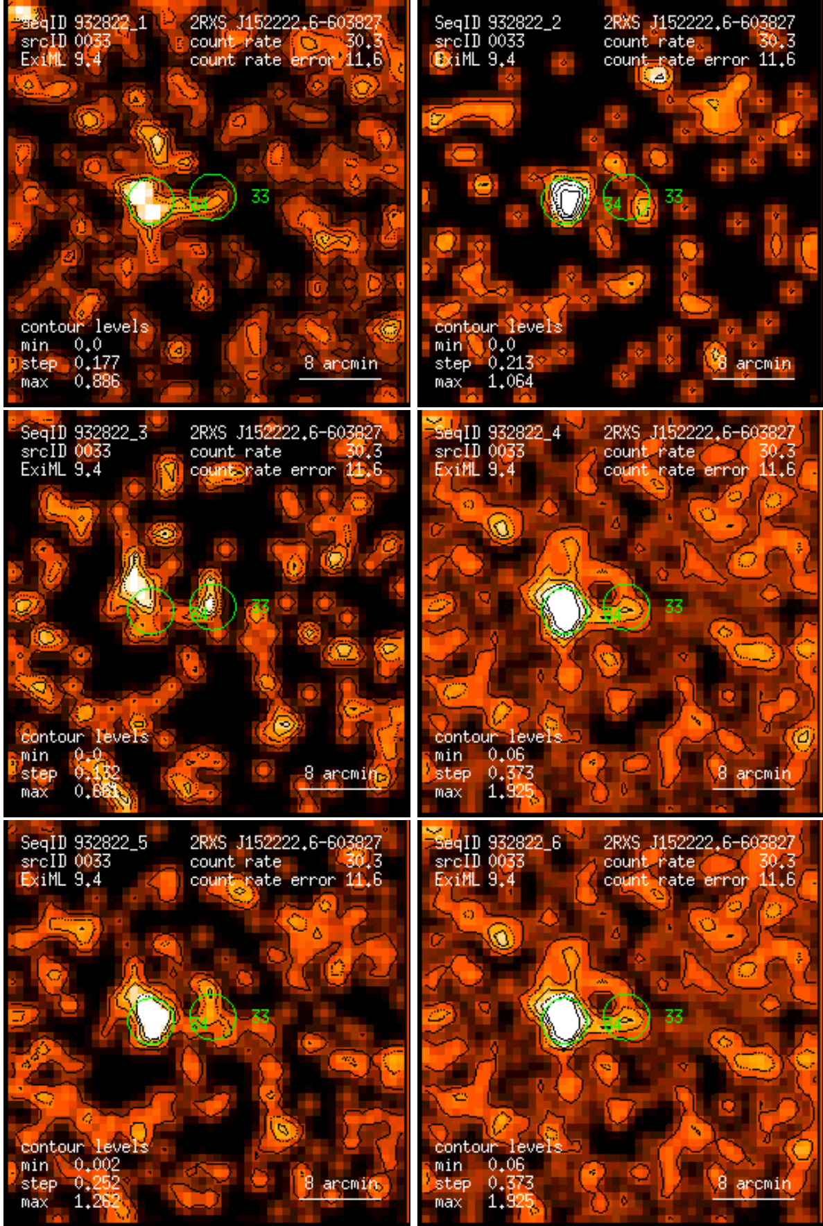
Figure 33: RASS 932822: detection 0033: band rate images, Gaussian filter: (1) PSPC channels 11 – 41, (2) 52 – 90, (3) 91 – 201, (4) 11 – 235, (5) 52 – 201, (6) 11 – 201. Broad band rates in counts/ks. Band rate contour levels in counts/ks/arcmin 2 .
