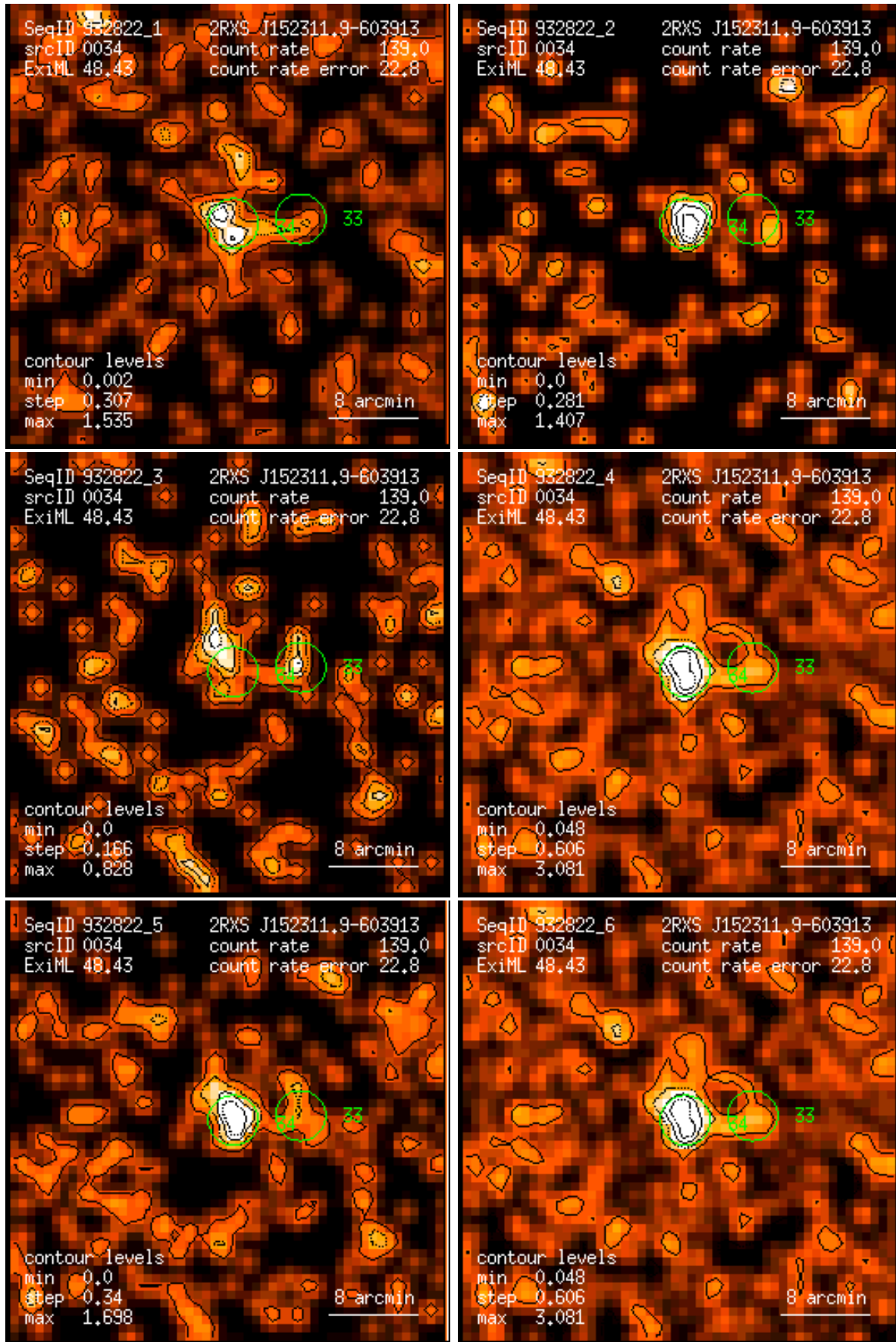
Figure 34: RASS 932822: detection 0034: band rate images, Gaussian filter: (1) PSPC channels 11 – 41, (2) 52 – 90, (3) 91 – 201, (4) 11 – 235, (5) 52 – 201, (6) 11 – 201. Broad band rates in counts/ks. Band rate contour levels in counts/ks/arcmin 2 .
