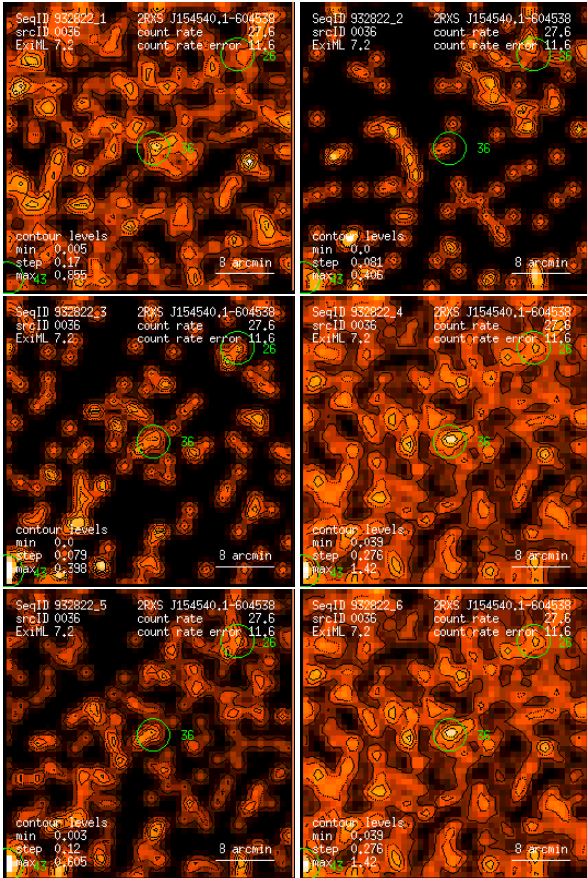
Figure 36: RASS 932822: detection 0036: band rate images, Gaussian filter: (1) PSPC channels 11 – 41, (2) 52 – 90, (3) 91 – 201, (4) 11 – 235, (5) 52 – 201, (6) 11 – 201. Broad band rates in counts/ks. Band rate contour levels in counts/ks/arcmin 2 .
