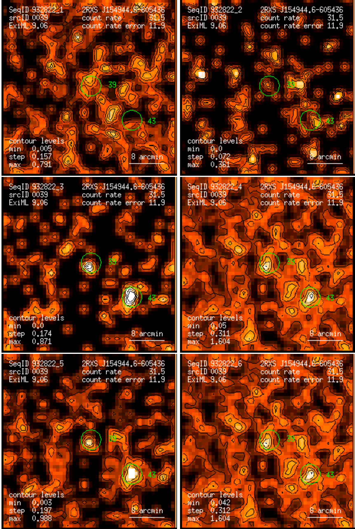
Figure 39: RASS 932822: detection 0039: band rate images, Gaussian filter: (1) PSPC channels 11 – 41, (2) 52 – 90, (3) 91 – 201, (4) 11 – 235, (5) 52 – 201, (6) 11 – 201. Broad band rates in counts/ks. Band rate contour levels in counts/ks/arcmin 2 .
