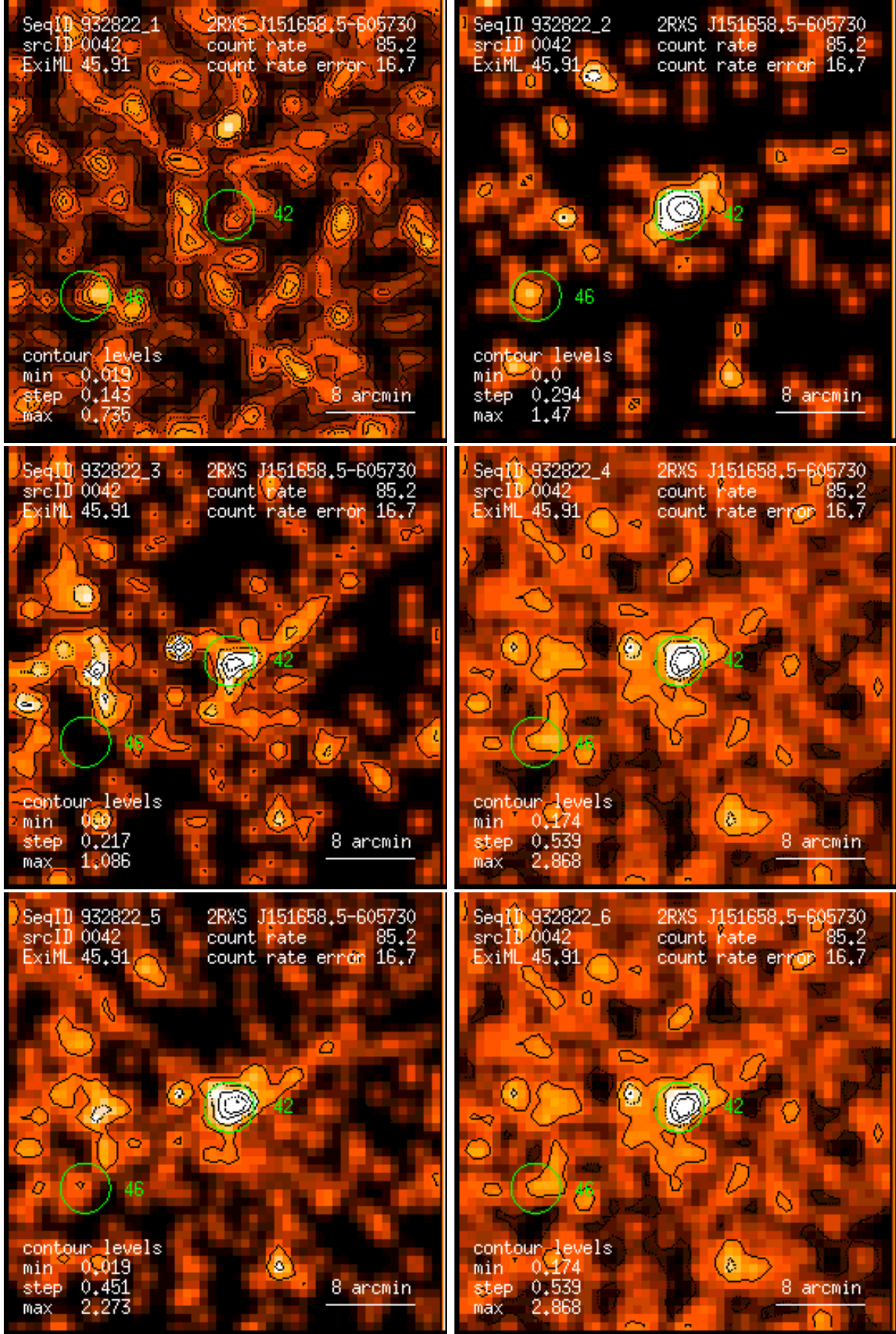
Figure 42: RASS 932822: detection 0042: band rate images, Gaussian filter: (1) PSPC channels 11 – 41, (2) 52 – 90, (3) 91 – 201, (4) 11 – 235, (5) 52 – 201, (6) 11 – 201. Broad band rates in counts/ks. Band rate contour levels in counts/ks/arcmin 2 .
