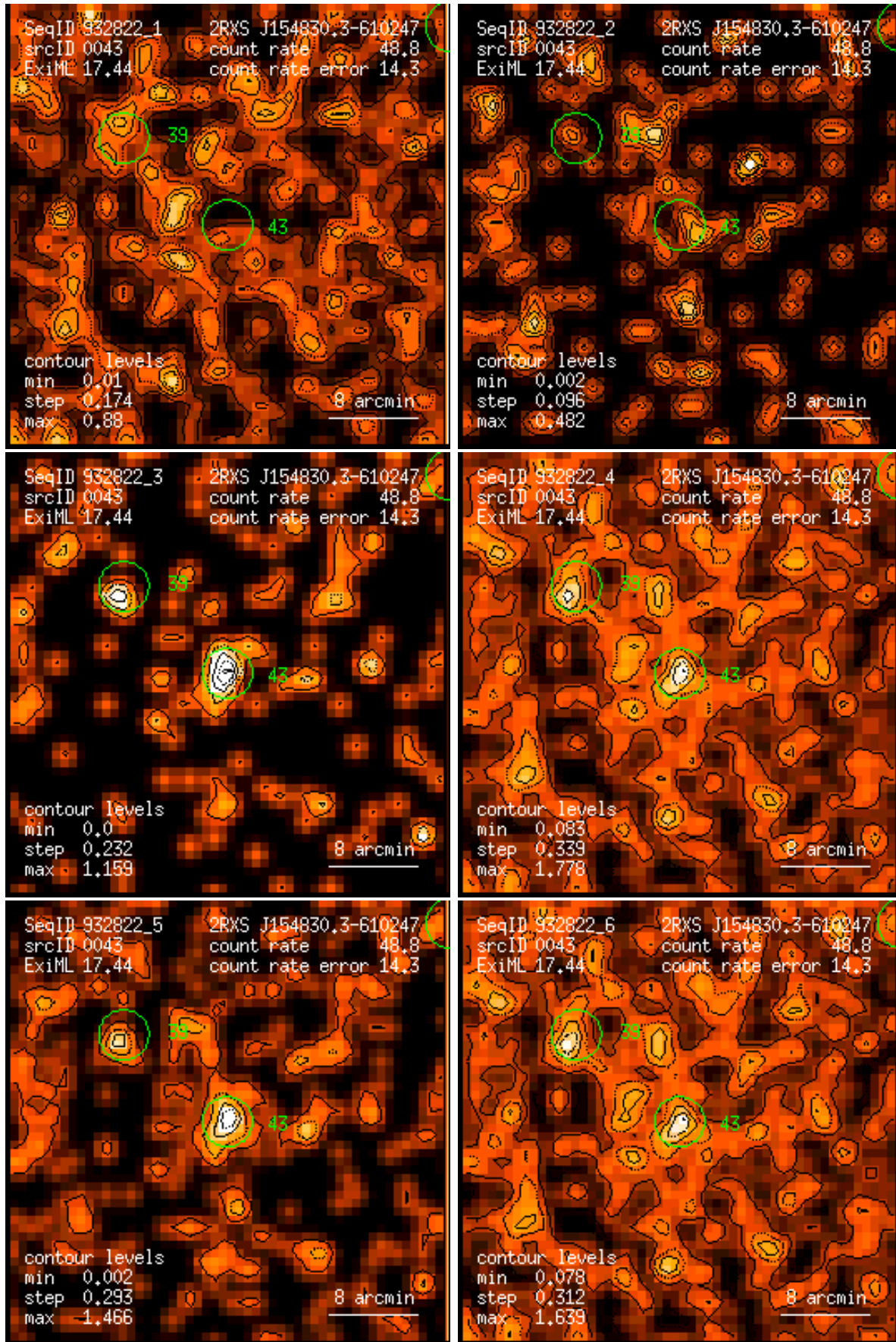
Figure 43: RASS 932822: detection 0043: band rate images, Gaussian filter: (1) PSPC channels 11 – 41, (2) 52 – 90, (3) 91 – 201, (4) 11 – 235, (5) 52 – 201, (6) 11 – 201. Broad band rates in counts/ks. Band rate contour levels in counts/ks/arcmin 2 .
