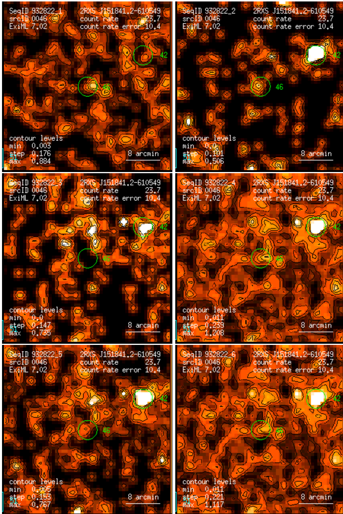
Figure 46: RASS 932822: detection 0046: band rate images, Gaussian filter: (1) PSPC channels 11 – 41, (2) 52 – 90, (3) 91 – 201, (4) 11 – 235, (5) 52 – 201, (6) 11 – 201. Broad band rates in counts/ks. Band rate contour levels in counts/ks/arcmin 2 .
