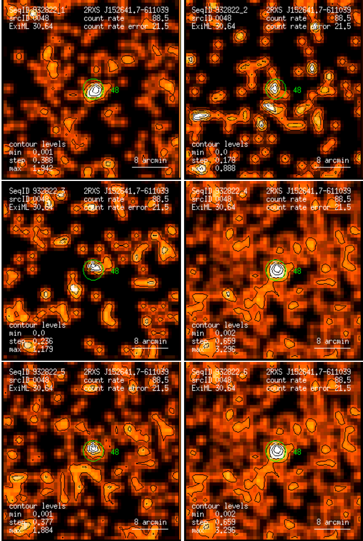
Figure 48: RASS 932822: detection 0048: band rate images, Gaussian filter: (1) PSPC channels 11 – 41, (2) 52 – 90, (3) 91 – 201, (4) 11 – 235, (5) 52 – 201, (6) 11 – 201. Broad band rates in counts/ks. Band rate contour levels in counts/ks/arcmin 2 .
