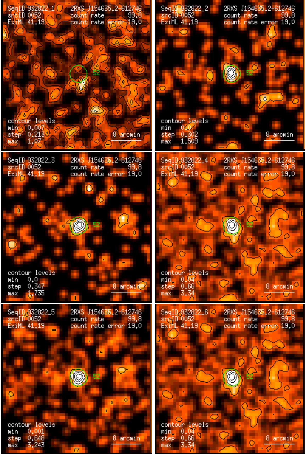
Figure 52: RASS 932822: detection 0052: band rate images, Gaussian filter: (1) PSPC channels 11 – 41, (2) 52 – 90, (3) 91 – 201, (4) 11 – 235, (5) 52 – 201, (6) 11 – 201. Broad band rates in counts/ks. Band rate contour levels in counts/ks/arcmin 2 .
