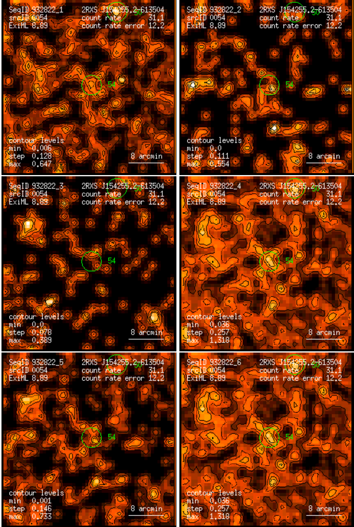
Figure 54: RASS 932822: detection 0054: band rate images, Gaussian filter: (1) PSPC channels 11 – 41, (2) 52 – 90, (3) 91 – 201, (4) 11 – 235, (5) 52 – 201, (6) 11 – 201. Broad band rates in counts/ks. Band rate contour levels in counts/ks/arcmin 2 .
