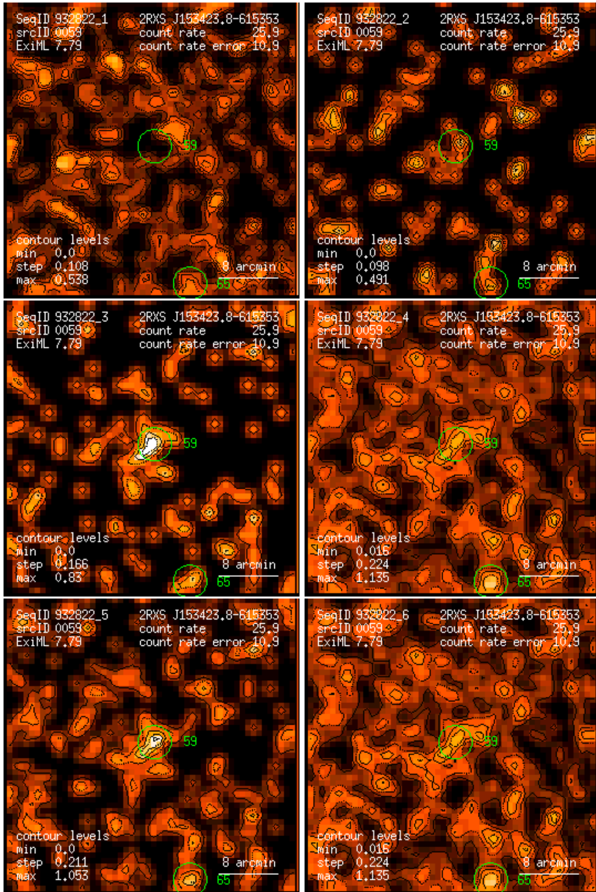
Figure 59: RASS 932822: detection 0059: band rate images, Gaussian filter: (1) PSPC channels 11 – 41, (2) 52 – 90, (3) 91 – 201, (4) 11 – 235, (5) 52 – 201, (6) 11 – 201. Broad band rates in counts/ks. Band rate contour levels in counts/ks/arcmin 2 .
