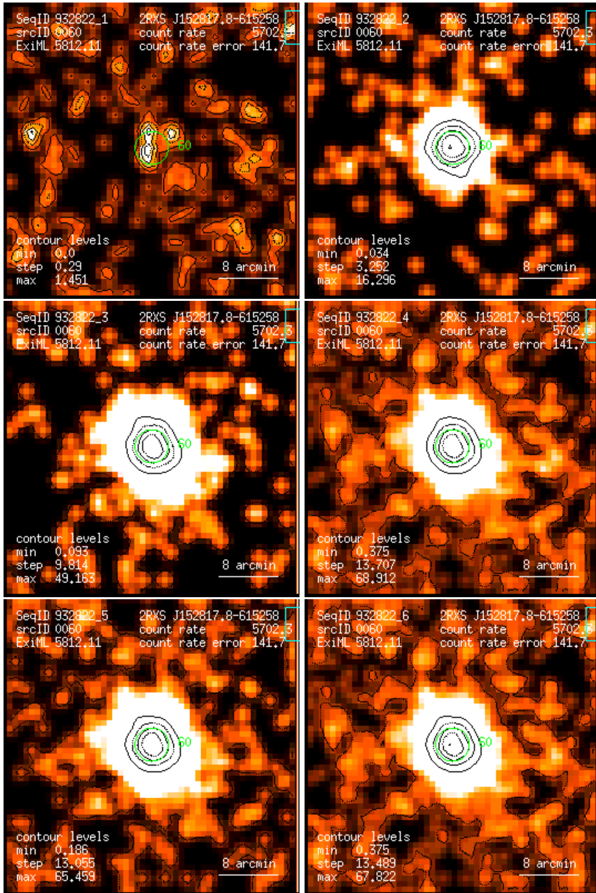
Figure 60: RASS 932822: detection 0060: band rate images, Gaussian filter: (1) PSPC channels 11 – 41, (2) 52 – 90, (3) 91 – 201, (4) 11 – 235, (5) 52 – 201, (6) 11 – 201. Broad band rates in counts/ks. Band rate contour levels in counts/ks/arcmin 2 .
