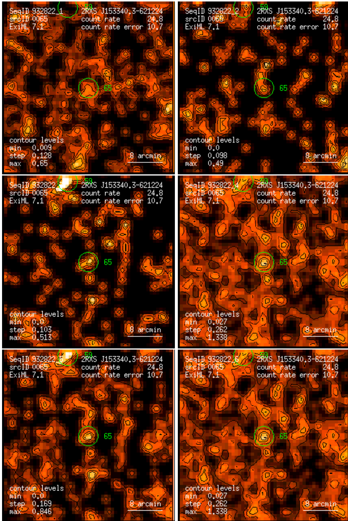
Figure 65: RASS 932822: detection 0065: band rate images, Gaussian filter: (1) PSPC channels 11 – 41, (2) 52 – 90, (3) 91 – 201, (4) 11 – 235, (5) 52 – 201, (6) 11 – 201. Broad band rates in counts/ks. Band rate contour levels in counts/ks/arcmin 2 .
