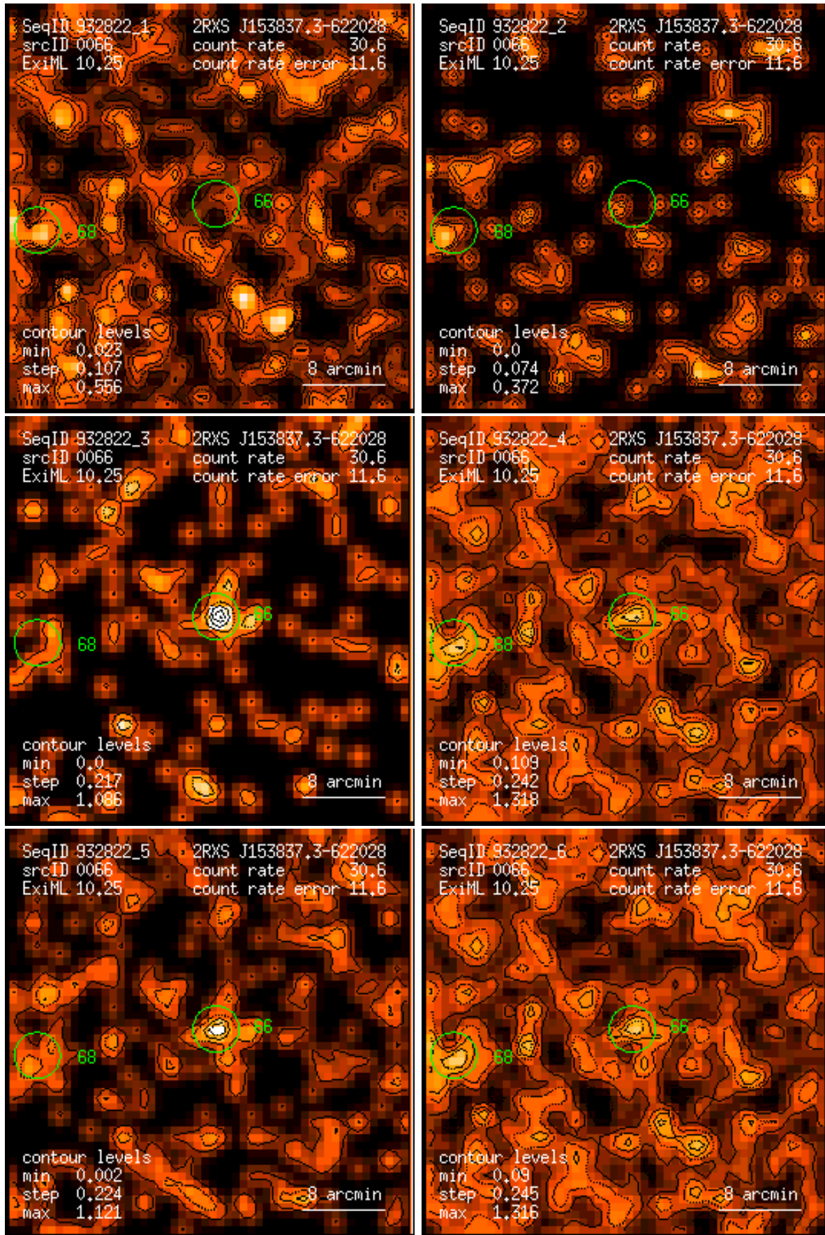
Figure 66: RASS 932822: detection 0066: band rate images, Gaussian filter: (1) PSPC channels 11 – 41, (2) 52 – 90, (3) 91 – 201, (4) 11 – 235, (5) 52 – 201, (6) 11 – 201. Broad band rates in counts/ks. Band rate contour levels in counts/ks/arcmin 2 .
