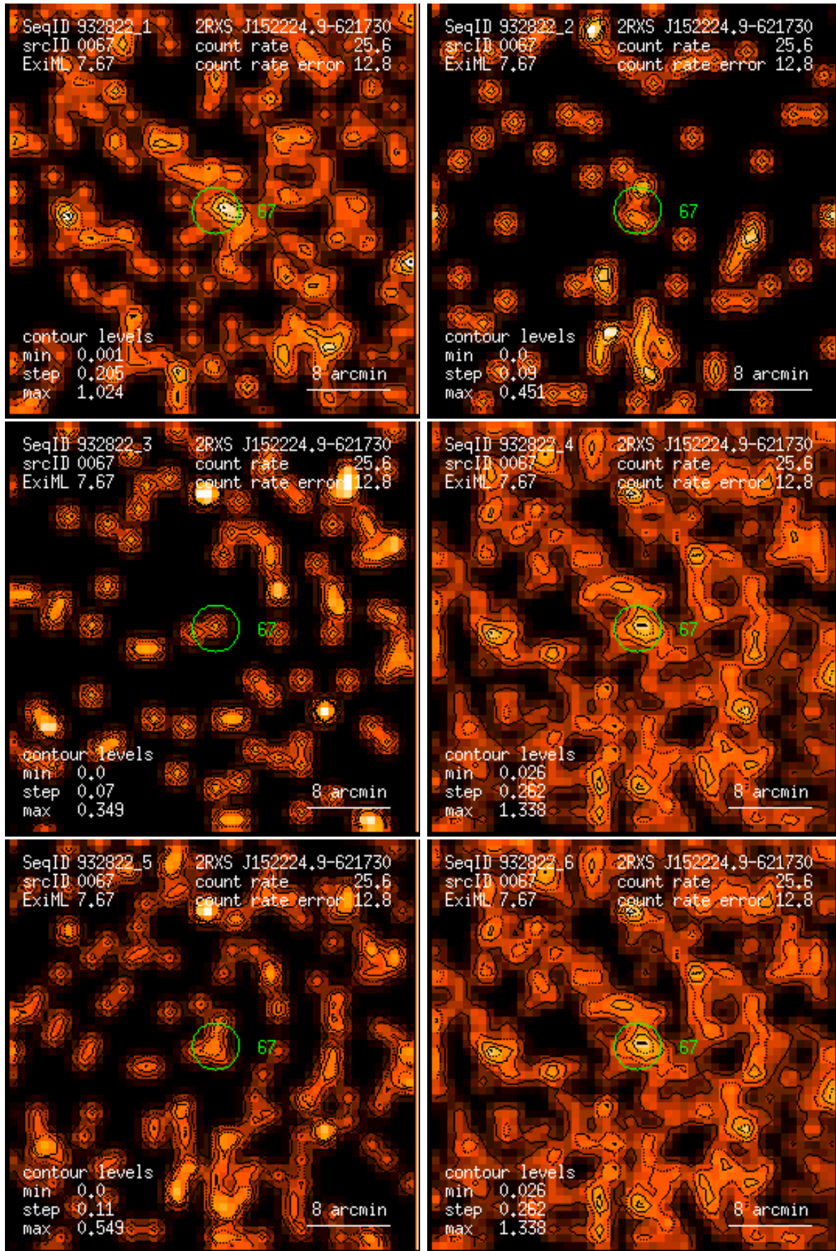
Figure 67: RASS 932822: detection 0067: band rate images, Gaussian filter: (1) PSPC channels 11 – 41, (2) 52 – 90, (3) 91 – 201, (4) 11 – 235, (5) 52 – 201, (6) 11 – 201. Broad band rates in counts/ks. Band rate contour levels in counts/ks/arcmin 2 .
