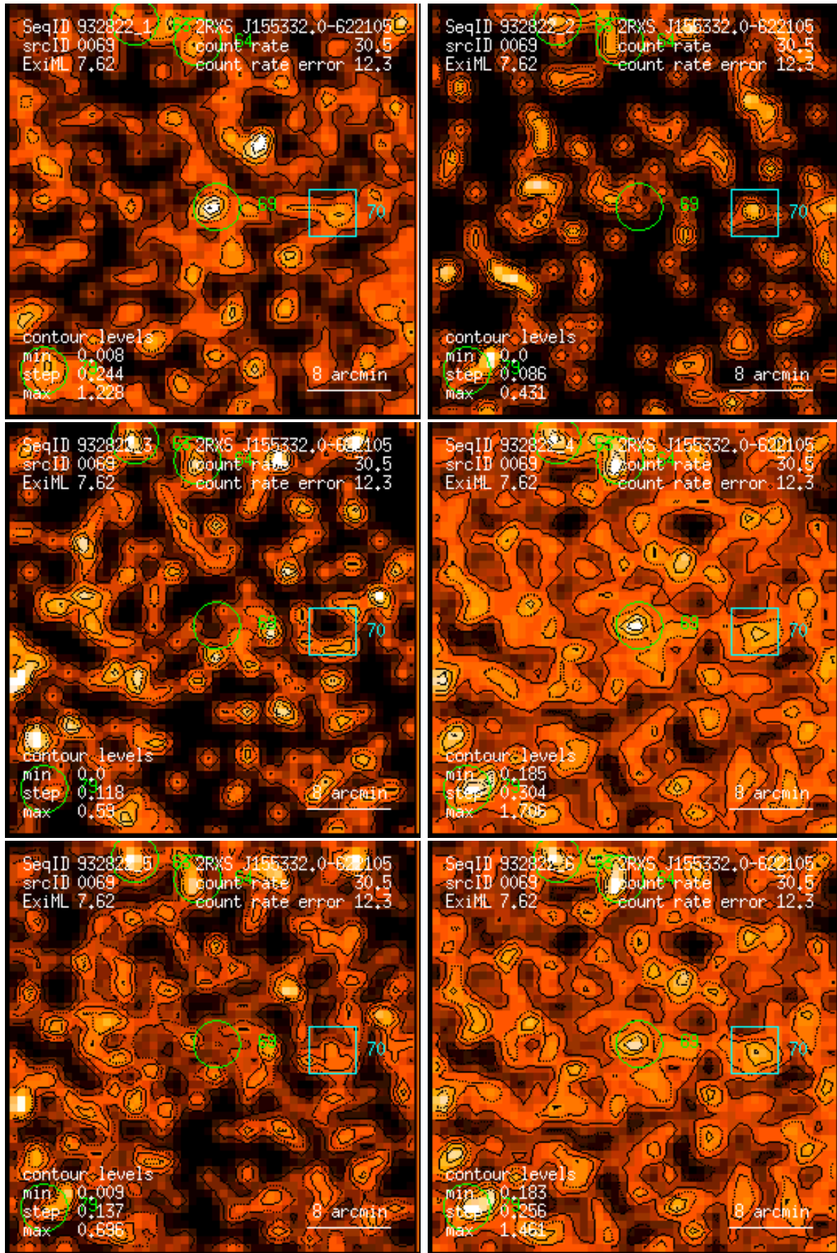
Figure 69: RASS 932822: detection 0069: band rate images, Gaussian filter: (1) PSPC channels 11 – 41, (2) 52 – 90, (3) 91 – 201, (4) 11 – 235, (5) 52 – 201, (6) 11 – 201. Broad band rates in counts/ks. Band rate contour levels in counts/ks/arcmin 2 .
