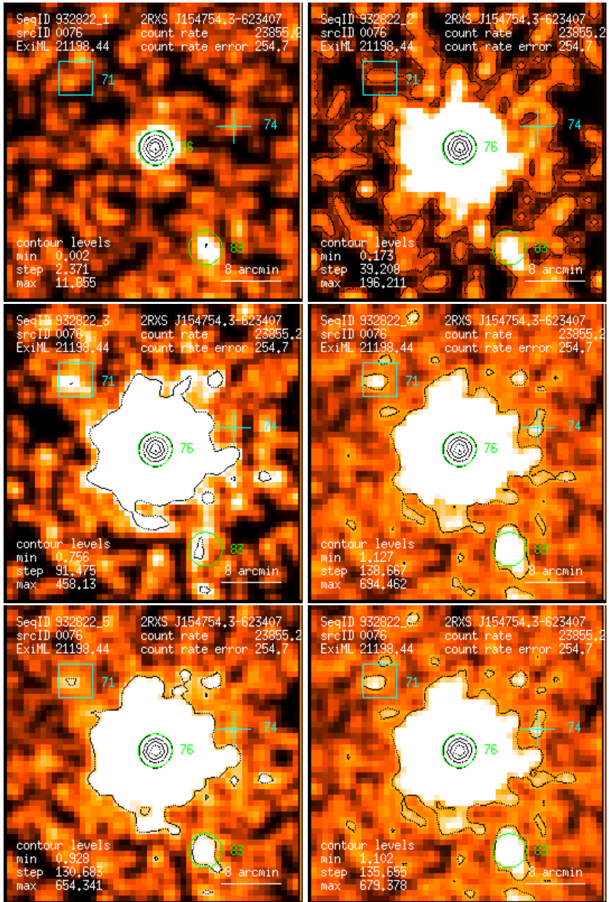
Figure 76: RASS 932822: detection 0076: band rate images, Gaussian filter: (1) PSPC channels 11 – 41, (2) 52 – 90, (3) 91 – 201, (4) 11 – 235, (5) 52 – 201, (6) 11 – 201. Broad band rates in counts/ks. Band rate contour levels in counts/ks/arcmin 2 .
