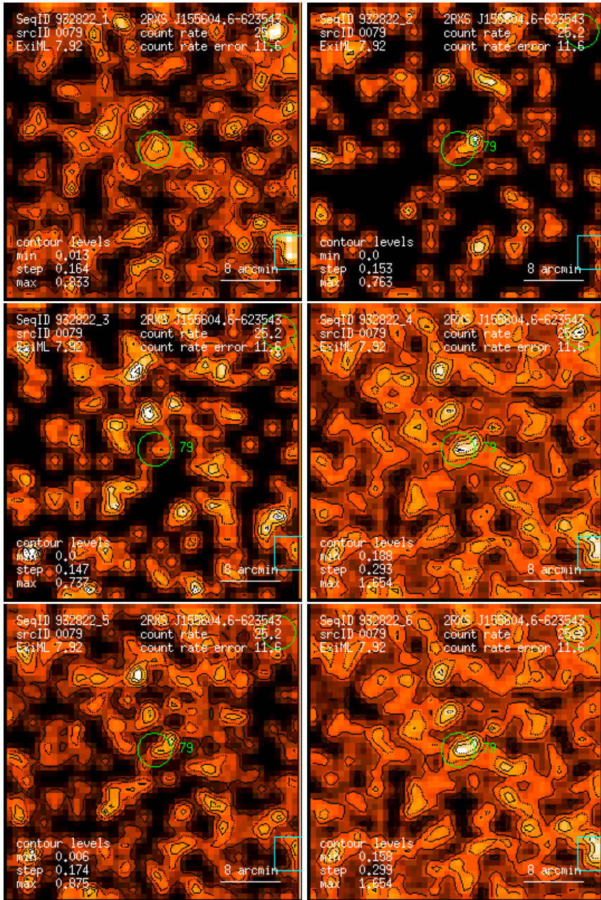
Figure 79: RASS 932822: detection 0079: band rate images, Gaussian filter: (1) PSPC channels 11 – 41, (2) 52 – 90, (3) 91 – 201, (4) 11 – 235, (5) 52 – 201, (6) 11 – 201. Broad band rates in counts/ks. Band rate contour levels in counts/ks/arcmin 2 .
