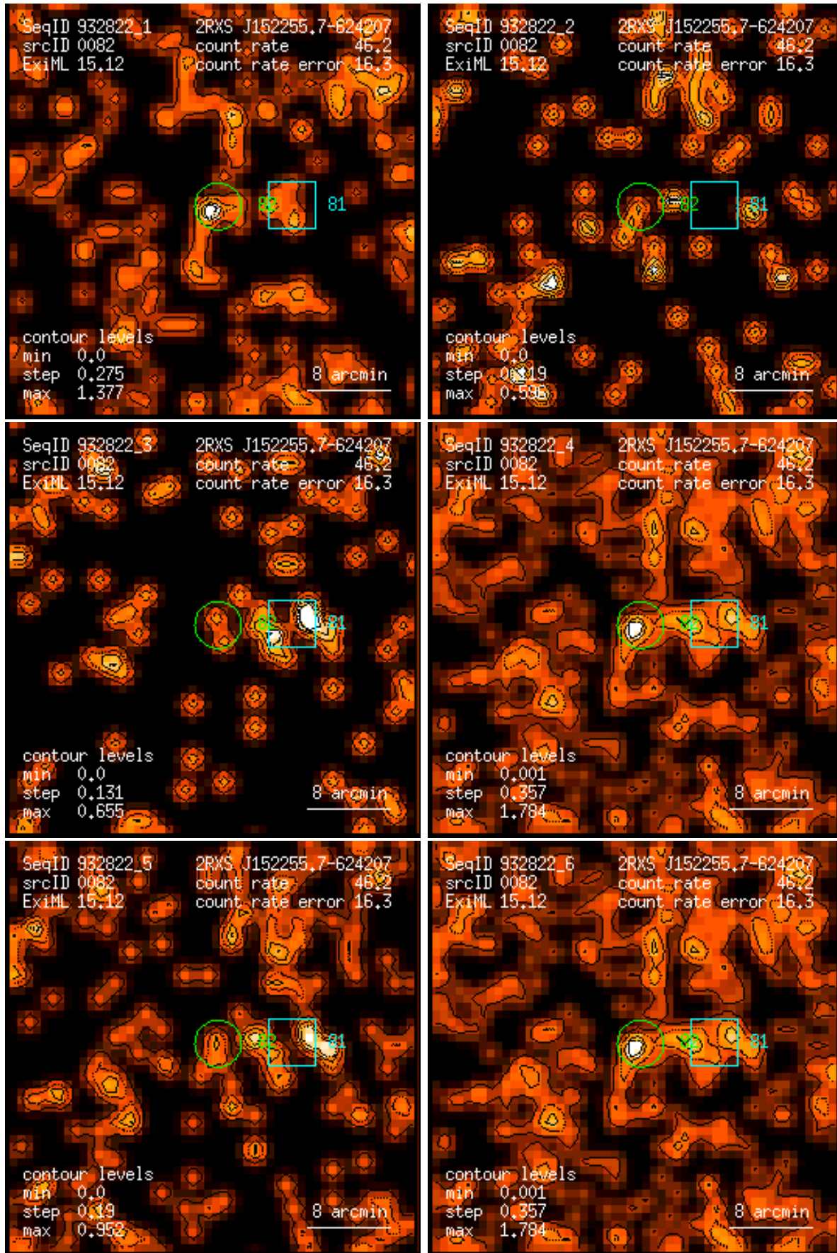
Figure 82: RASS 932822: detection 0082: band rate images, Gaussian filter: (1) PSPC channels 11 – 41, (2) 52 – 90, (3) 91 – 201, (4) 11 – 235, (5) 52 – 201, (6) 11 – 201. Broad band rates in counts/ks. Band rate contour levels in counts/ks/arcmin 2 .
