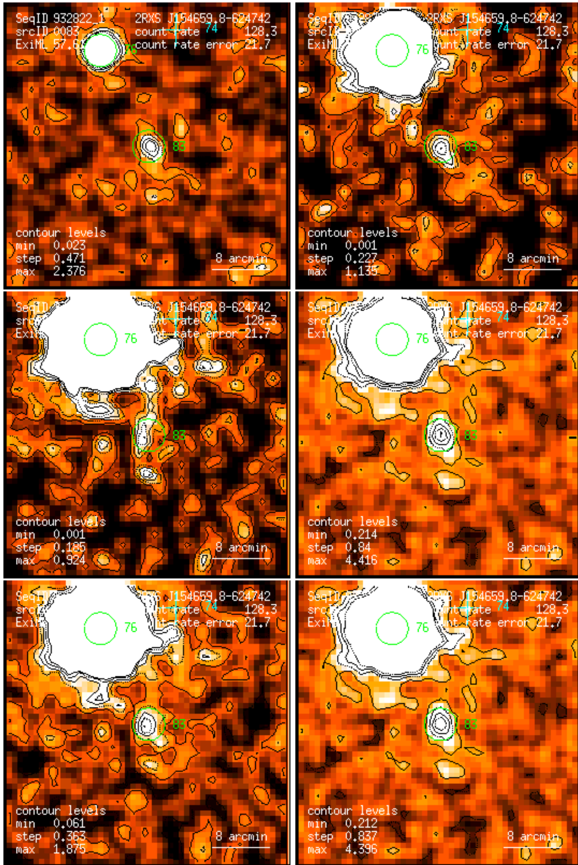
Figure 83: RASS 932822: detection 0083: band rate images, Gaussian filter: (1) PSPC channels 11 – 41, (2) 52 – 90, (3) 91 – 201, (4) 11 – 235, (5) 52 – 201, (6) 11 – 201. Broad band rates in counts/ks. Band rate contour levels in counts/ks/arcmin 2 .
