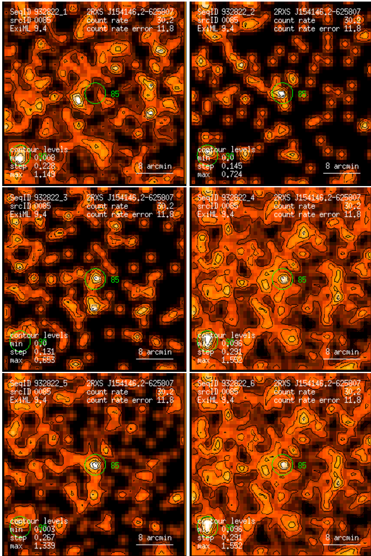
Figure 85: RASS 932822: detection 0085: band rate images, Gaussian filter: (1) PSPC channels 11 – 41, (2) 52 – 90, (3) 91 – 201, (4) 11 – 235, (5) 52 – 201, (6) 11 – 201. Broad band rates in counts/ks. Band rate contour levels in counts/ks/arcmin 2 .
