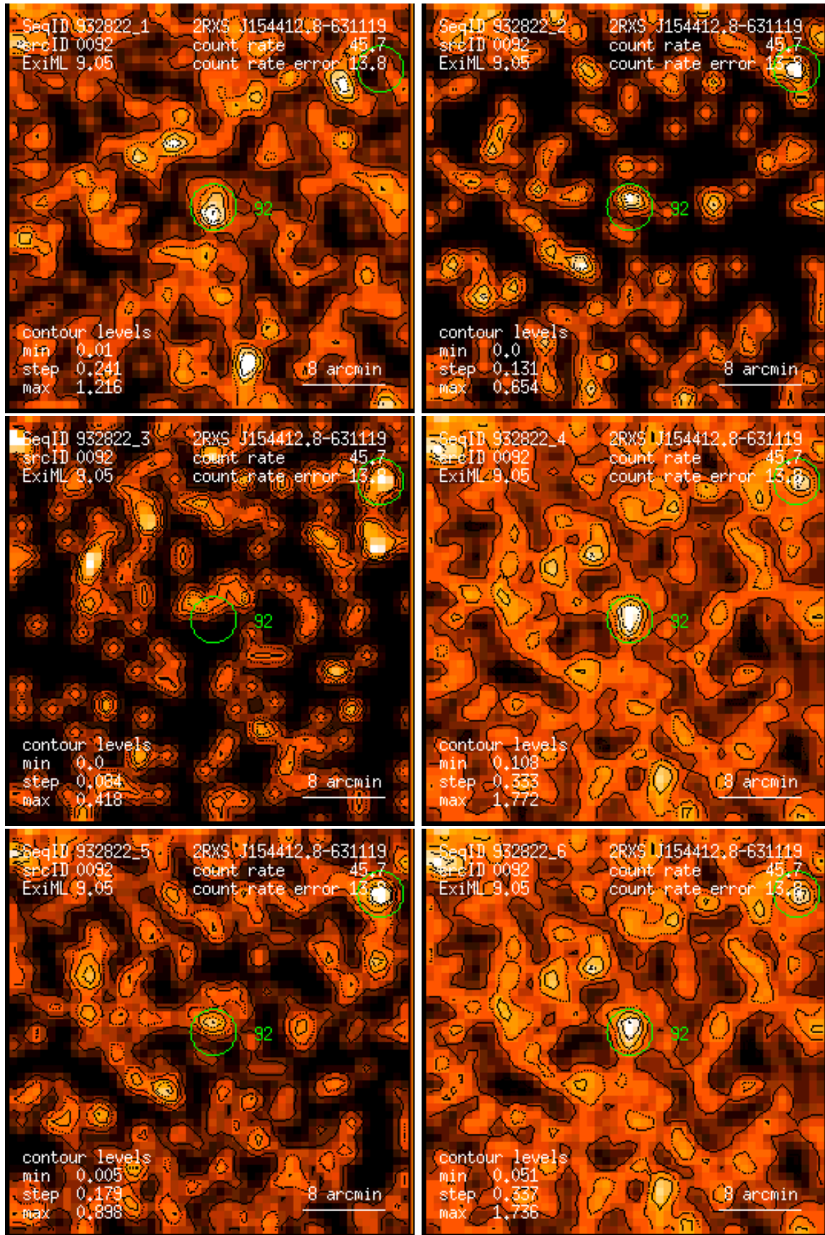
Figure 92: RASS 932822: detection 0092: band rate images, Gaussian filter: (1) PSPC channels 11 – 41, (2) 52 – 90, (3) 91 – 201, (4) 11 – 235, (5) 52 – 201, (6) 11 – 201. Broad band rates in counts/ks. Band rate contour levels in counts/ks/arcmin 2 .
