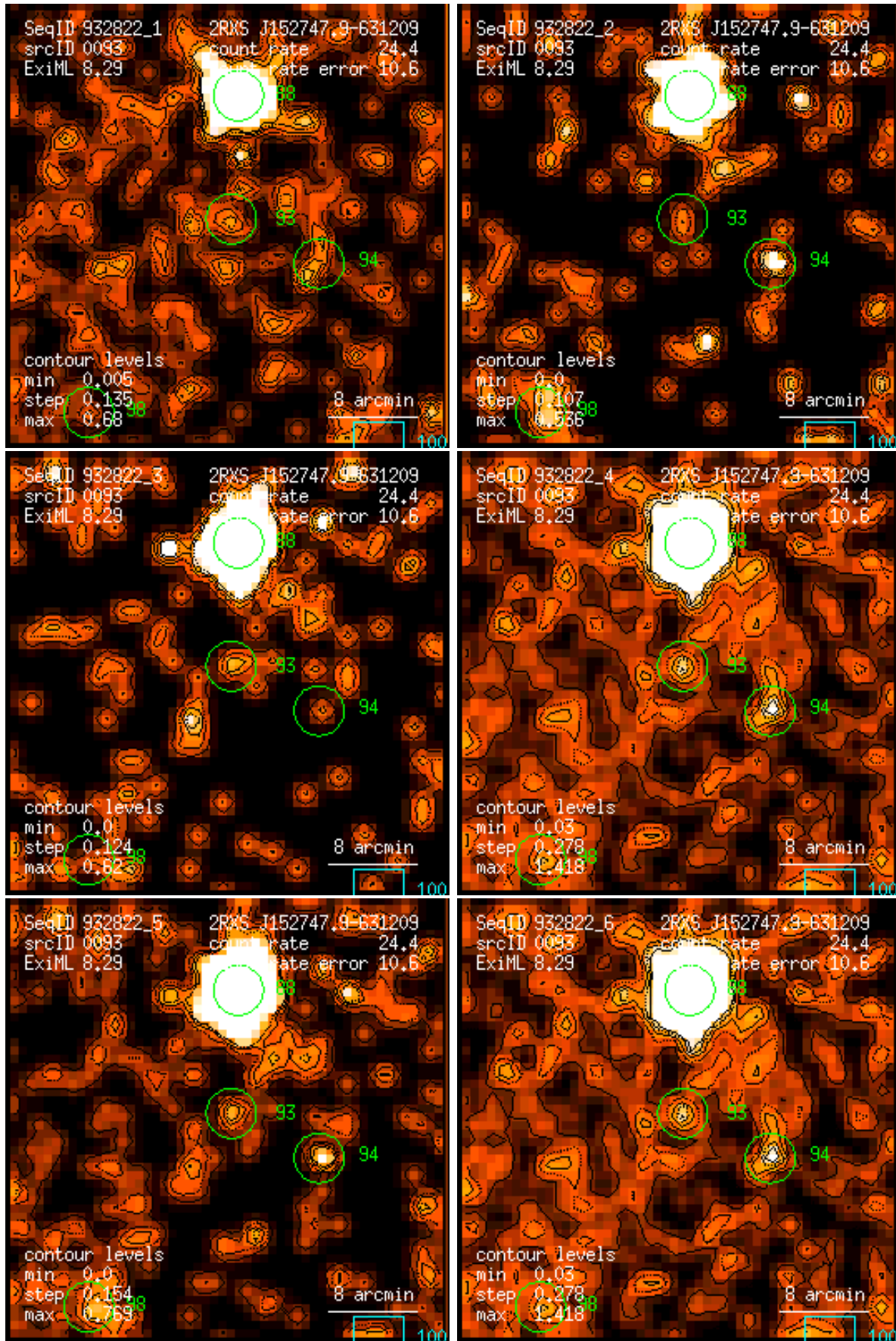
Figure 93: RASS 932822: detection 0093: band rate images, Gaussian filter: (1) PSPC channels 11 – 41, (2) 52 – 90, (3) 91 – 201, (4) 11 – 235, (5) 52 – 201, (6) 11 – 201. Broad band rates in counts/ks. Band rate contour levels in counts/ks/arcmin 2 .
